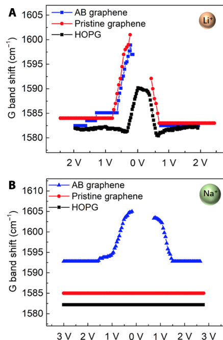
Fig. 4. Comparison of \text{Li}^+ and \text{Na}^+ intercalation in different materials. (A) Shift of G band position during \text{Li}^+ intercalation taking place in all materials tested: HOPG, graphene, and AB graphene. (B) Same experiment performed with \text{Na}^+ , showing no intercalation for HOPG and graphene, but intercalation in AB graphene. Some experimental points in the range around 0 V are not reported because the G band decreased so much that it was not possible to measure precisely its shift.
