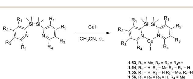
Scheme 9 Synthesis of complexes 1.53–56.
