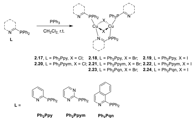
Scheme 20 Synthesis of 2.17–24 .
