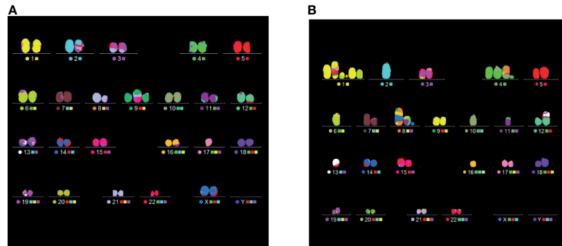
FIGURE 11 | Examples of CA analysis by mFISH. Images depict karyotypes from samples irradiated at the CNAO beamline with 4 Gy of protons in the presence of BSH and show typical aberrations types found at two positions, i.e. a simple exchange between chromosomes 2 and 17 from a cell exposed at the entrance [left panel, (A) ] and several complex rearrangement detected in a PCC spread from a cell irradiated at the distal position [right panel, (B) ]. See main text for details.
