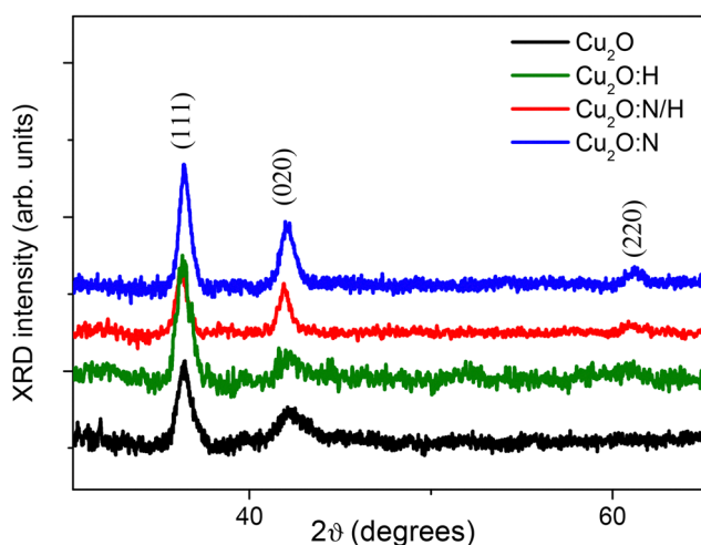
Fig. 2 XRD Diffractograms of Cu 2 O films. Miller indexes correspond to the cubic Cu 2 O phase.
