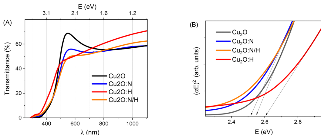
Fig. 1 (A) UV-vis-NIR transmittance spectra against the photon wavelength, \lambda (and the photon energy, E ), and (B) Tauc plot against the photon energy, E , of pure and doped Cu 2 O films. The arrows indicate the estimated optical band gaps (the band gap values are basically identical for the Cu 2 O:N and Cu 2 O:N/H samples).
