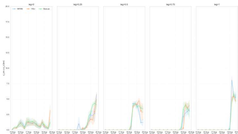
Figure 20. Vertical moment ( z_{cm} + \sigma_z ) of the tracer column along the transect for tr17_t3 (legs 0, 0.25, 0.5, 0.75, and 1). The curves indicating MYNN, YSU, and BouLac.
