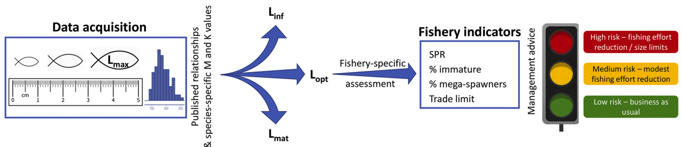
Fig. 1. Schematic of the different steps to be followed to apply the literature-based method to assess stock status with only available information the maximum length (L max ) and length-frequency distribution. L inf : asymptotic size, L opt : optimum harvest size, L mat : size at maturity, SPR: spawning potential ratio.
