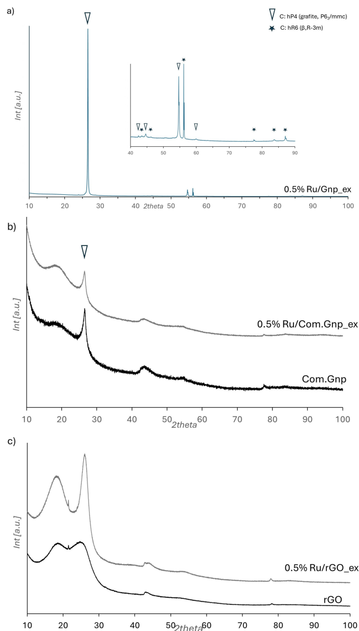
Figure 8. XRD patterns of Ru-based catalysts: (a) 0.5% Ru/Gnp pattern - in the inset, the pattern is shown with an enlarged intensity scale; (b) 0.5% Ru/Com.Gnp ex and its bare support; (c) 0.5% Ru/rGO ex and the corresponding support.
