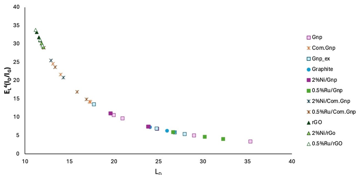
Figure 10. Number of defects as a function of the distance of defect L_D [nm] for the investigated catalytic materials after CO 2 hydrogenation reaction.
