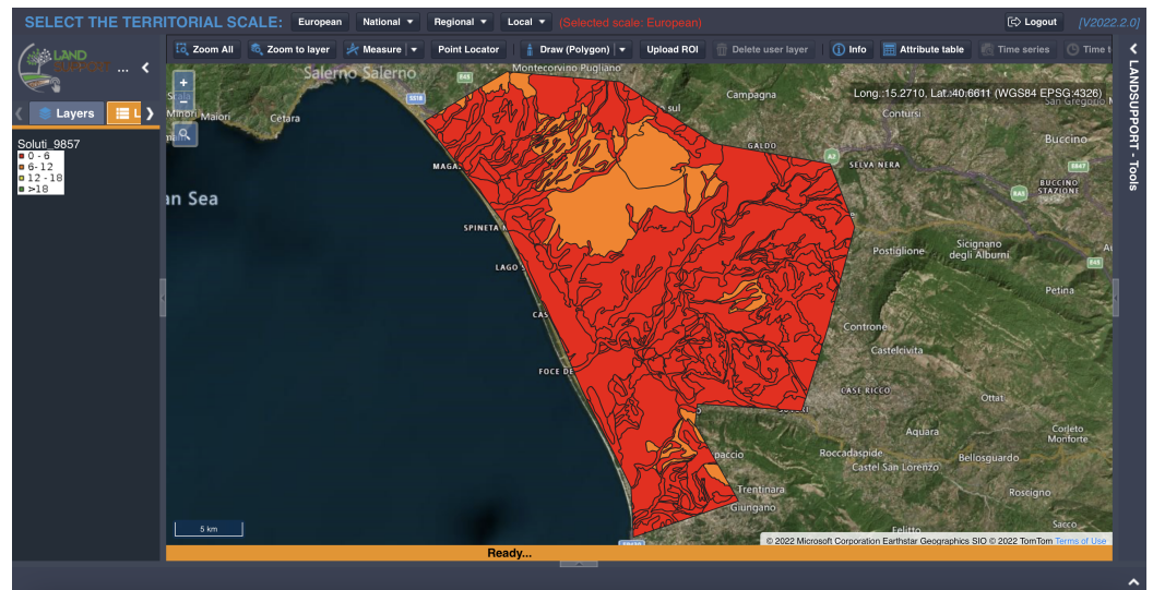
Figure 6. Nitrate fate tool application in a ROI drawn in the Piana del Sele, simulating the rotation tomato–alfalfa, with inorganic fertilization, irrigation at 100% of the crop demand, minimum tillage and retained residue. The legend, in the left panel of the LS GUI, helps with the interpretation of the map colours.
