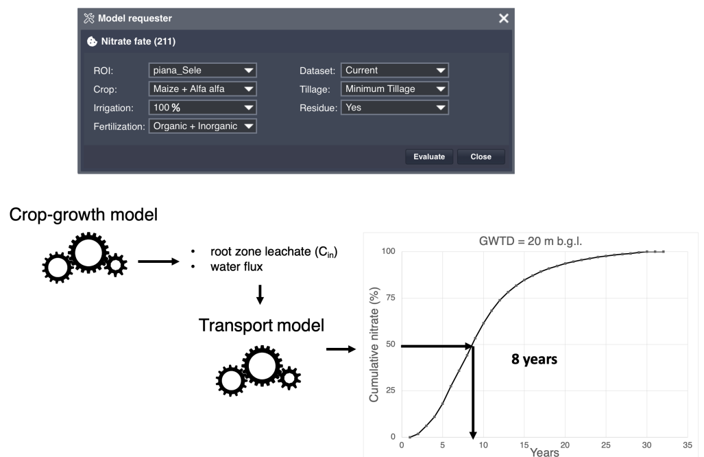
Figure 4. Workflow of the coupling of the ARMOSA and TFM-ext models, starting from the end-user requests. The out-to-in connections allow the evaluation of the cumulative nitrate leachate at the groundwater table depth and the time for the 50% arrival.
