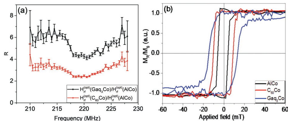
Figure 4. a) Ratio R of the optimal rf field of the Co/molecule systems ( H_{\text{rf}}^{\text{(opt)}}(X) ) divided by the optimal rf field of the reference sample ( H_{\text{rf}}^{\text{(opt)}}(\text{Al}) ), proportional to the ratio between the mean enhancement factor of the Co/molecule system and the corresponding of the reference sample. b) L-MOKE normalized hysteresis loops at 77 K for Gaq 3 -Co and C 60 -Co. The applied field direction is the same as the rf field in NMR experiments.
