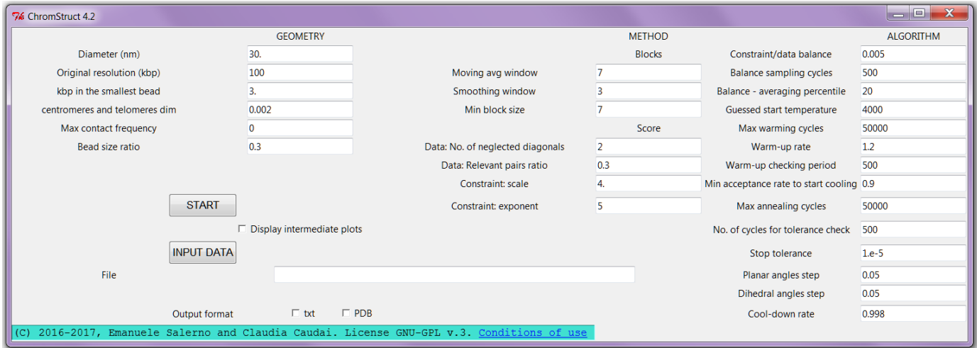
Fig. 5. CHROMSTRUCT 4.2 Graphical User Interface. All the parameters are set at their default values.
