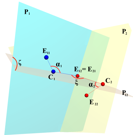
Fig. 1. Two adjacent beads represented as centroid-endpoint triples. E_{11} , E_{21} : endpoints “1” of beads 1 and 2. E_{12} , E_{22} : endpoints “2” of beads 1 and 2. C_1 , C_2 : centroids of beads 1 and 2. P_1 , P_2 : planes spanned by beads 1 and 2. P_{12} : plane spanned by the triple C_1 - E_{12} - C_2 . \alpha_1 , \alpha_2 : inner angles (fixed). \xi : planar angle. \zeta : dihedral angle.
