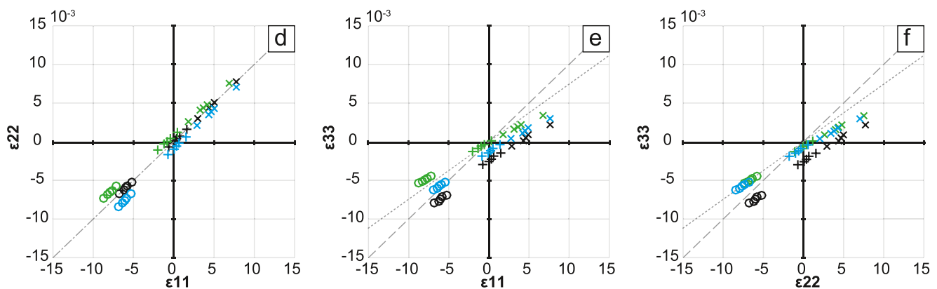
Figure 5. Plots of the relaxed anisotropic linear strains ( \epsilon_{11} , \epsilon_{22} , and \epsilon_{33} ) within quartz inclusions contained in the zircon hosts for multiple sets of entrapment conditions and crystallographic orientations (RCO). Within each set of entrapment conditions, the strains of five P - T points were calculated. The dashed gray lines represent the strains calculated from hydrostatic conditions and isotropic strains.
