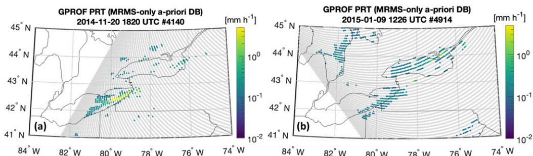
FIG. 12. Maps of GPROF estimates made forcing the GV-MRMS-only a priori database for (a) orbit 4140 and for (b) orbit 4914.
