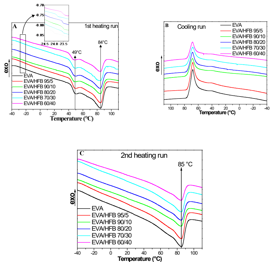
Figure 2. DSC curves of EVA and its composites: (A) first run from -40 °C to 120 °C; (B) cooling run from 120 °C to -40 °C; and (C) second heating run from -40 °C to 120 °C (heat flow rate: 10 °C/min).
