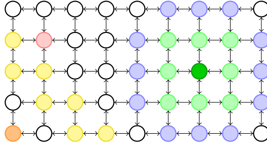
Figure 1: Example of spatial properties. The orange point satisfies \diamond_{[3,5]} pink . The orange point satisfies \square_{[2,3]} yellow . All green points satisfy green \mathcal{S}_{[0,100]} blue . The dark green point satisfies also green \mathcal{S}_{[2,3]} blue .
