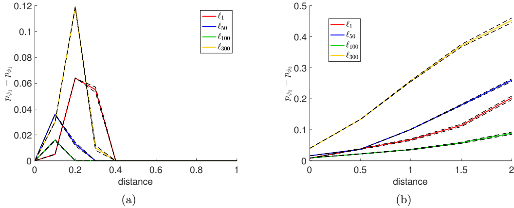
Figure 13: (a) p_{\psi_1} - p_{\phi_1} vs the distance d = [0, 1.0] (b) p_{\psi_3} - p_{\phi_3} vs the distance d = [0, 2.0] .
