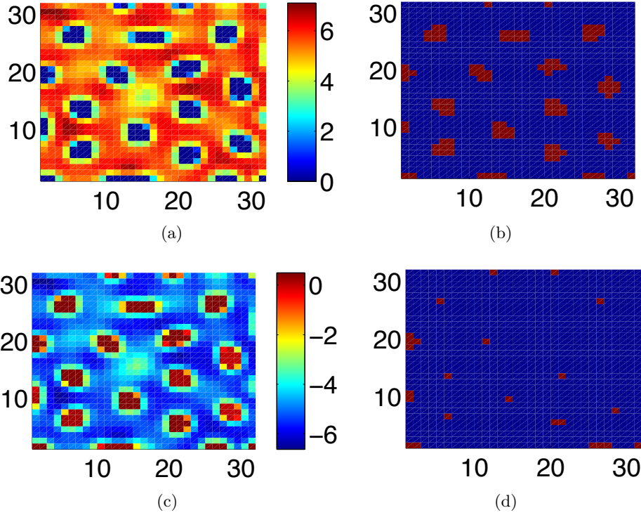
Figure 3: Satisfaction of formula (3.4) with h = 0.5 , T_{\text{pattern}} = 19 , \delta = 1 , T_{\text{end}} = 30 , d_1 = 1 , d_2 = 6 for (b), (c) and d_2 = 4 for (d). (a) Concentration of A at time t = 50 ; (b) (d) Boolean semantics of the property \varphi_{\text{spotFormation}} ; the cells (locations) that satisfy the formula are in red, the others are in blue; (c) Quantitative semantics of the property \varphi_{\text{spotFormation}} ; The value of the robustness is given by a colour map as specified in the legend on the right of the figure.
