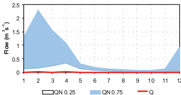
Fig. 6. Natural streamflow (25 th and 75 th percentiles) and actual monthly median streamflow (Q) at River Section 2.
