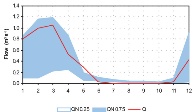
Fig. 5. Natural streamflow (25 th and 75 th percentiles) and actual monthly median streamflow (Q) at River Section 1.
