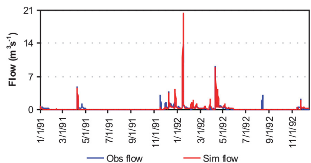
Fig. 2. Measured and simulated streamflow at gauge 1. Calibration (1991–1992).
