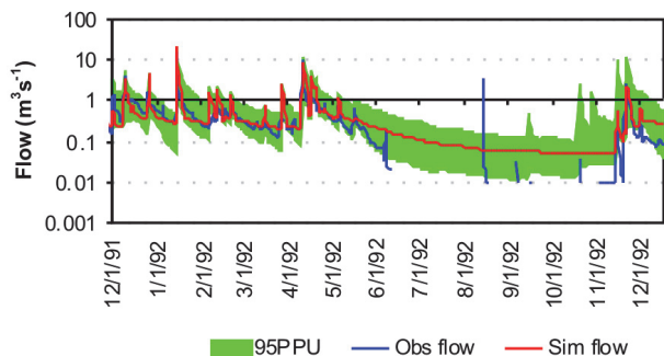
Fig. 4. Comparison of the hydrograph and uncertainty prediction at gauge 1. Obs flow represents measured discharge in impacted conditions and Sim flow represents the calibrated simulation in natural conditions. The shaded (green) interval is the 95% uncertainty predictions (P-factor = 0.41; and R-factor = 0.20).
