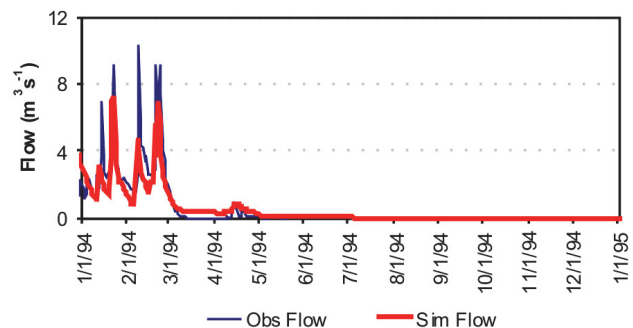
Fig. 3. Measured and simulated streamflow at gauge 2. Validation (1994).
