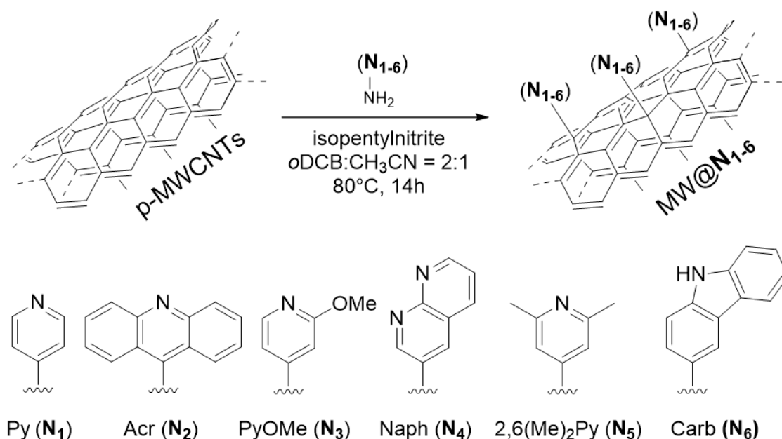
Scheme 1. Exohedrally N-decorated MWCNTs (MW@N 1-6 ) as metal free-catalysts for the CO 2 reduction reaction (CO 2 RR).
