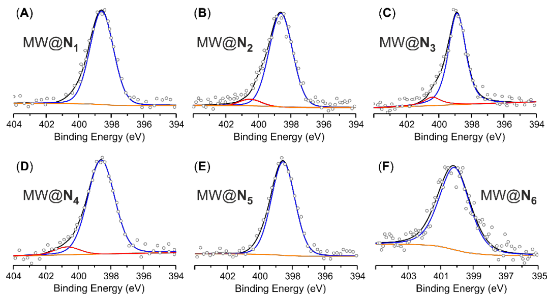
Figure 1. High resolution X-ray photoelectron spectroscopy (XPS) N 1s core level regions for samples MW@N 1 (A); MW@N 2 (B); MW@N 3 (C); MW@N 4 (D); MW@N 5 (E); MW@N 6 (F) along with their respective peak fittings.
