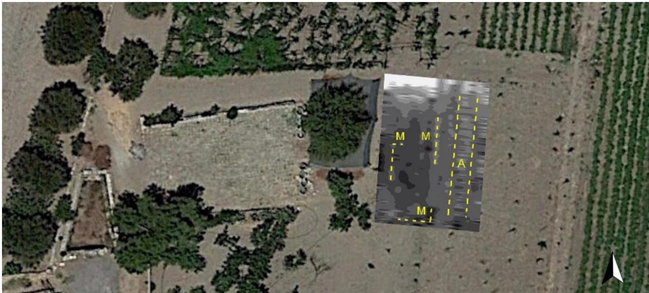
Fig. 4. Area M1: georeferenced gradiometric data.
