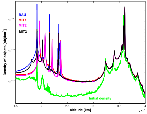
Figure 6. Density of objects larger than 10 cm in the BAU (blue line), MIT1 (red line), MIT2 (magenta line) and MIT3 (black line) cases, in the MEO and GEO region in the year 2205. The green line shows the initial (year 2005) density.
