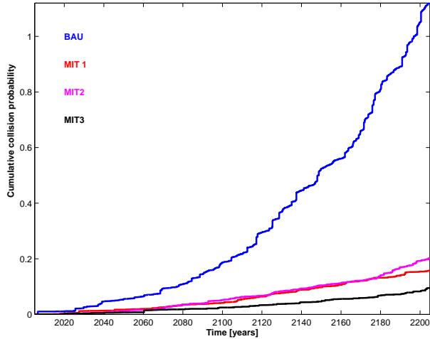
Figure 10. Expected cumulative number of collisions in the BAU (blue line), MIT1 (red line), MIT2 (magenta line) and MIT3 (black line) cases, in the MEO region.
