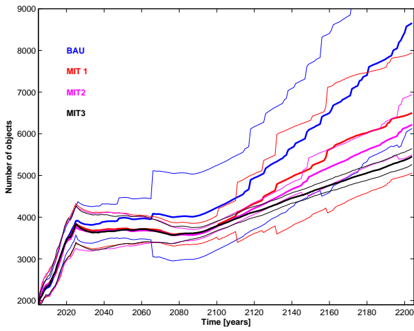
Figure 4. Effective number of objects larger than 10 cm in the BAU (blue line), MIT1 (red line), MIT2 (magenta line) and MIT3 (black line) cases in the MEO region. The thin lines are the plus or minus 1\sigma limits.
