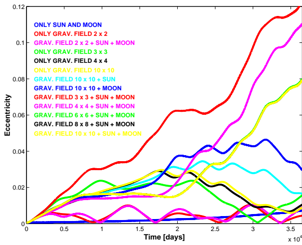
Figure 1. Resonance onset. Long term evolution of the orbital eccentricity for a GPS like orbit with increasingly complex perturbative models.
