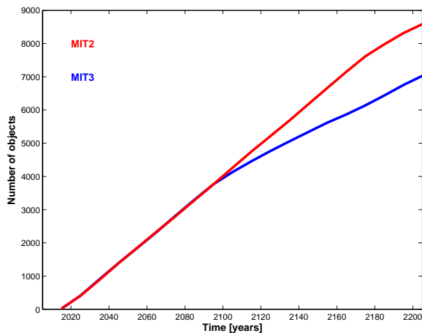
Figure 13. Number of disposed GALILEO satellites present in space as a function of time, in the MIT2 (red line) and MIT3 (blue line) cases, in all the 40 Monte Carlo runs. Note how, after about 80–90 years from the beginning of the simulation, the two lines start to diverge due to the reentry of the satellites disposed on initially eccentric orbits.
