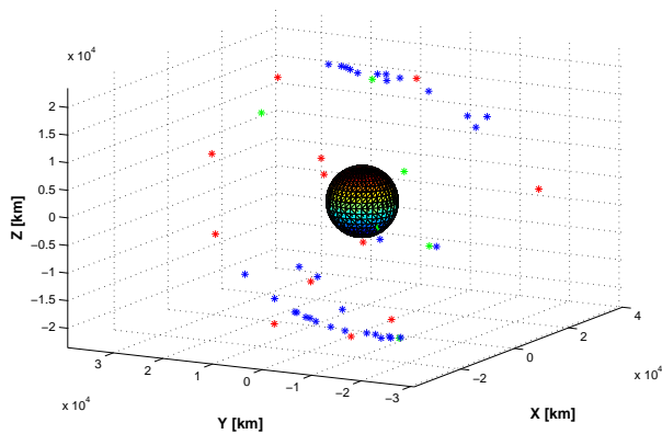
Figure 11. Location, in Earth centered Cartesian coordinates, of the collision induced breakups recorded in 40 Monte Carlo runs, involving at least one MEO object: BAU (blue asterisks), MIT1 (red asterisks), MIT2 (green asterisks).
