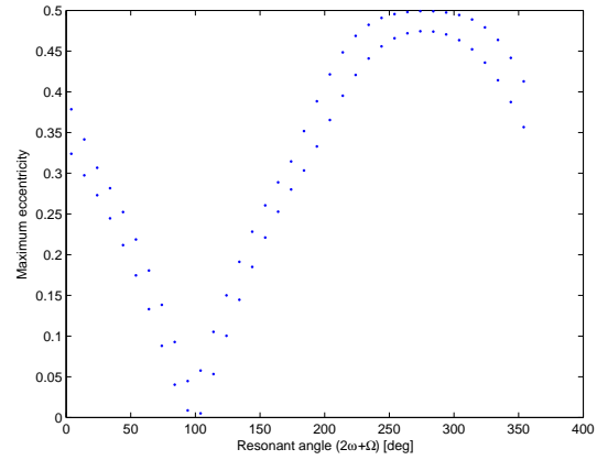
Figure 3. Maximum eccentricity growth, as a function of initial resonant argument 2\omega + \Omega , for a GPS disposal orbit.
