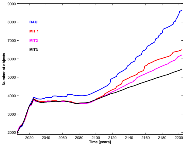
Figure 5. As in Fig. 4, but showing only the average values of the 40 Monte Carlo runs.
