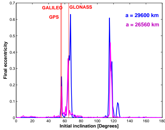
Figure 2. Maximum eccentricity growth after 200 years as a function of initial inclination for GALILEO-like (blue line) and GPS-like orbits (magenta line).
