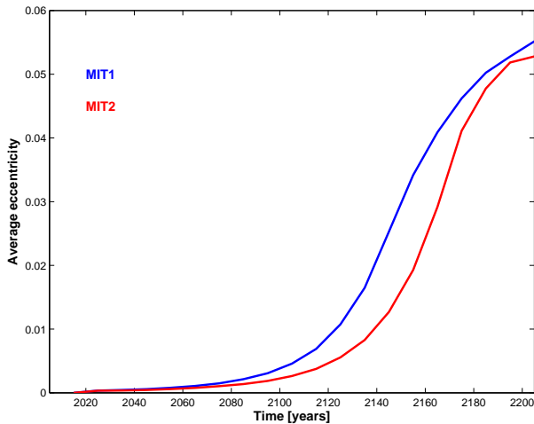
Figure 8. Time evolution of the average eccentricity of the orbits of all the disposed GALILEO satellites, from all the 40 Monte Carlo runs. The blue line refers to the MIT1 scenario and the red line to the MIT2 scenario.
