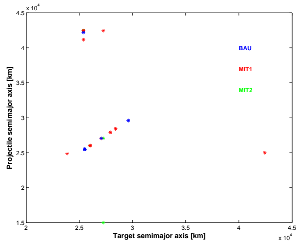
Figure 12. Semimajor axis of the targets and projectiles involved in all the MEO fragmentations recorded in the 40 Monte Carlo runs of the 4 cases. Note that, as explained in the text, no collision involving MEO objects is recorded in the MIT3 case and that several occurrences in the BAU case appear superimposed in the plot, around the GLONASS orbit semimajor axis.
