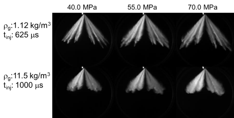
Figure 1. Liquid spray images at different injection pressures and ambient densities; T_{amb} : 20°C.
