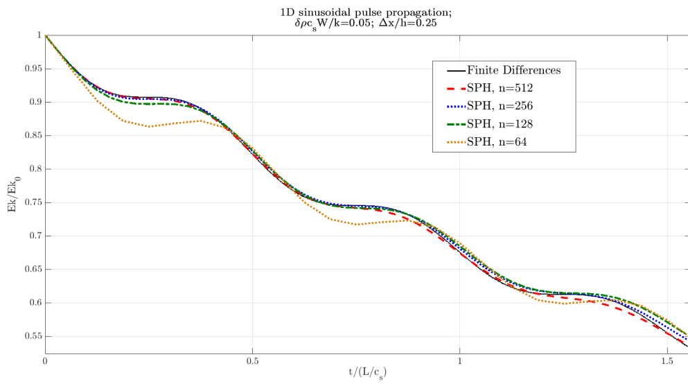
FIG. 3: Sinusoidal pulse. Kinetic energy; time history
