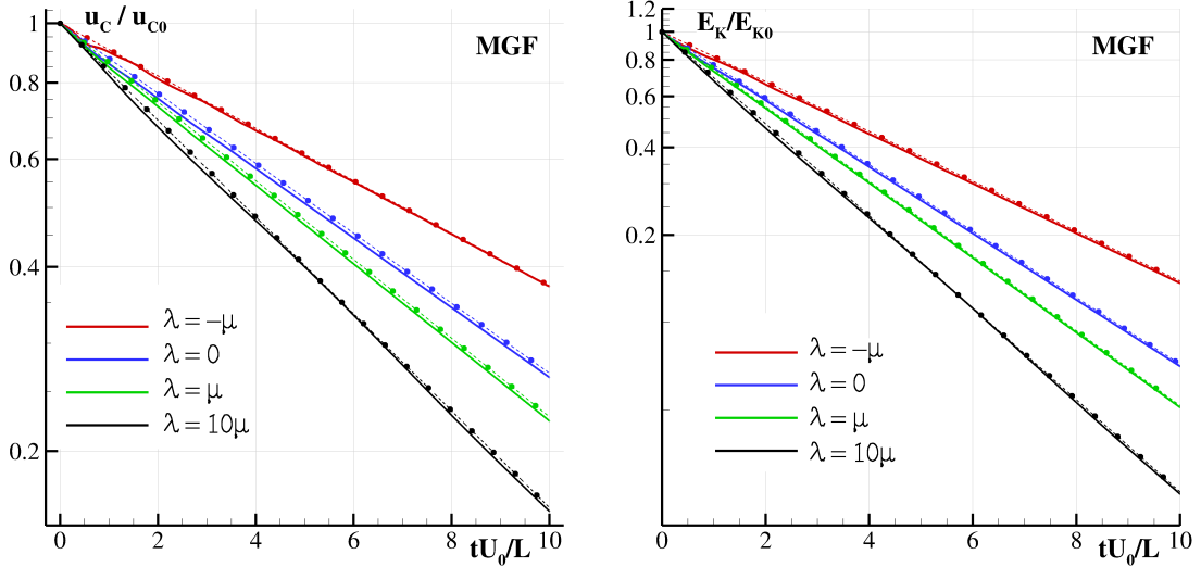
FIG. 5: Pipe flow: time decay of the velocity at the center of the fluid domain (left column) and of the total kinetic energy (right column) for different values of the ratio \sigma = \lambda/\mu . The dash-dotted lines represent the analytical solutions while the solid-line are the SPH solutions.
