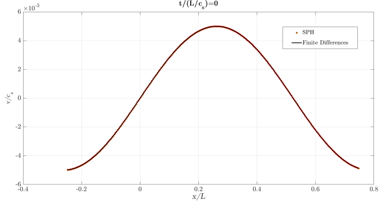
FIG. 1: Sinusoidal pulse. Initial velocity field, n = 256
