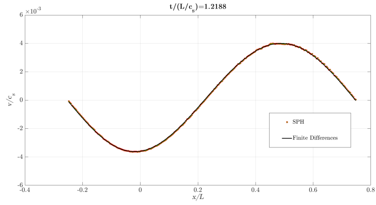
FIG. 2: Sinusoidal pulse. Velocity field, n = 256 , t/(L/c_s) \approx 1.22
