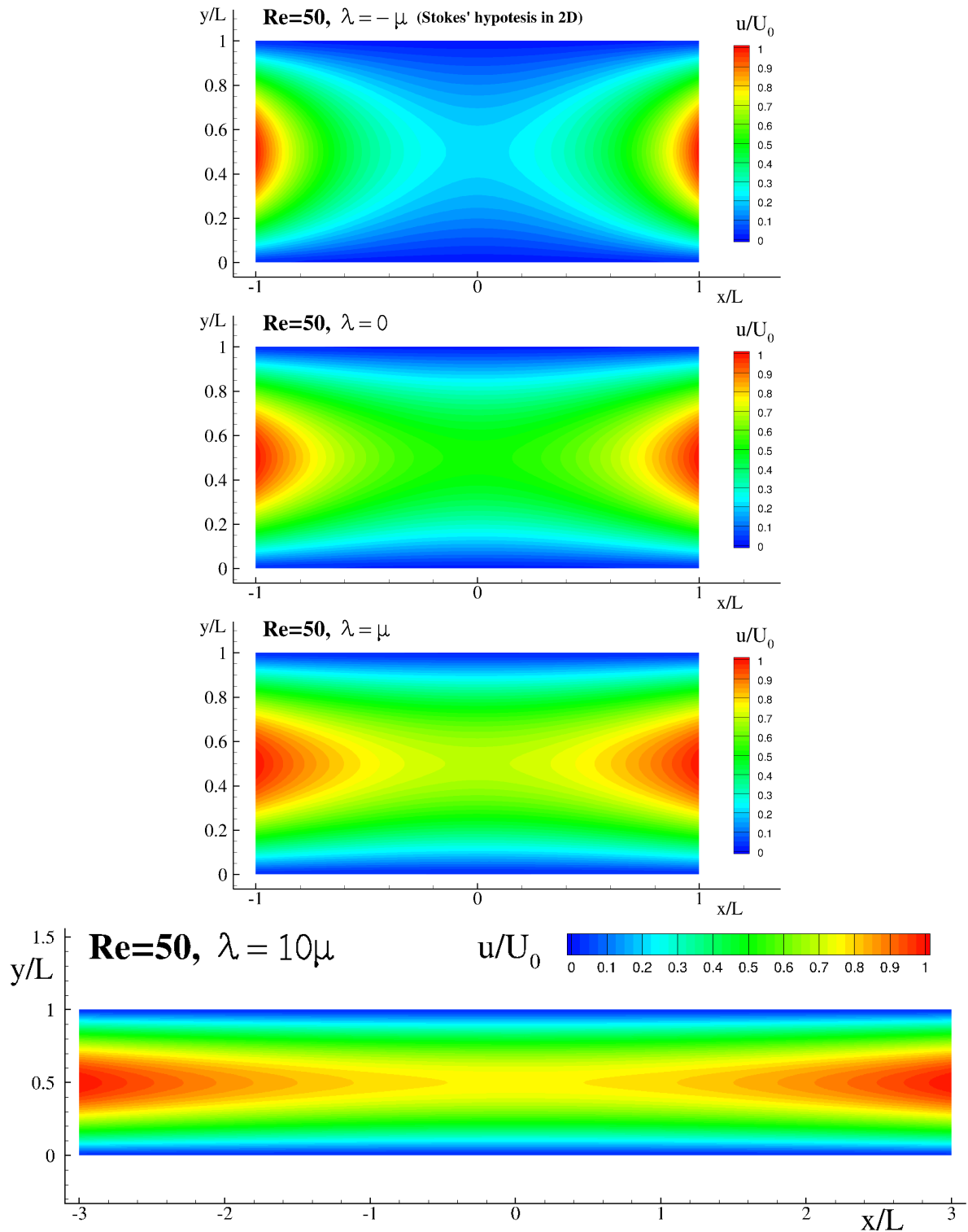
FIG. 4: Pipe flow: initial velocity field for different values of the ratio \sigma = \lambda/\mu .
