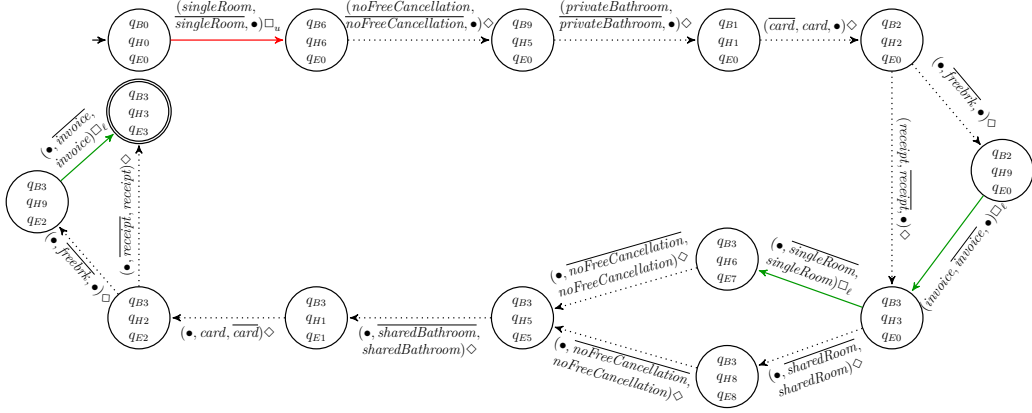
Figure 5: Orchestration of composition \text{BusinessClient} \otimes \text{Hotel} \otimes \text{EconomyClient} of the three automata in Figures 2, 3 and 4 for the product P4858
