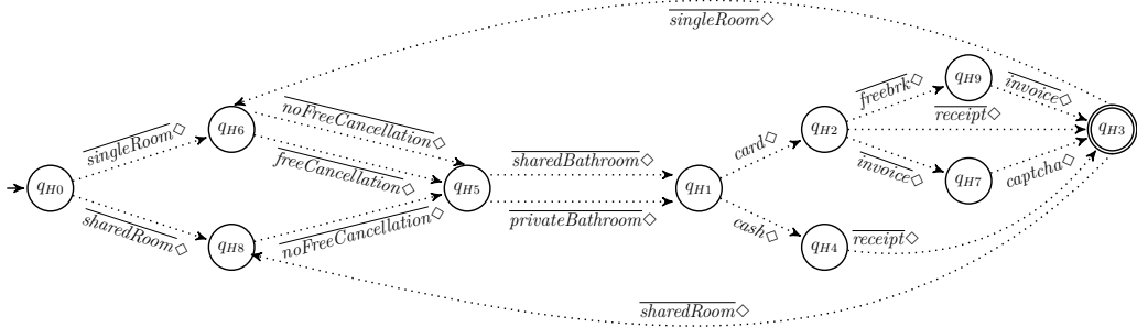
Figure 3: The automaton for Hotel
