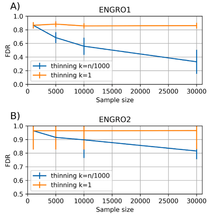
Fig. 1. Mean and standard deviation of the FDR across the 20 samples for the ENGRO1 (a) and ENGRO2 (b) metabolic models, considering 1000, 5000, 10 000 and 30 000 elements, without applying any thinning (i.e. k = 1 ) or with thinning k = n/1000 , where n is the dimension of the sample size.
