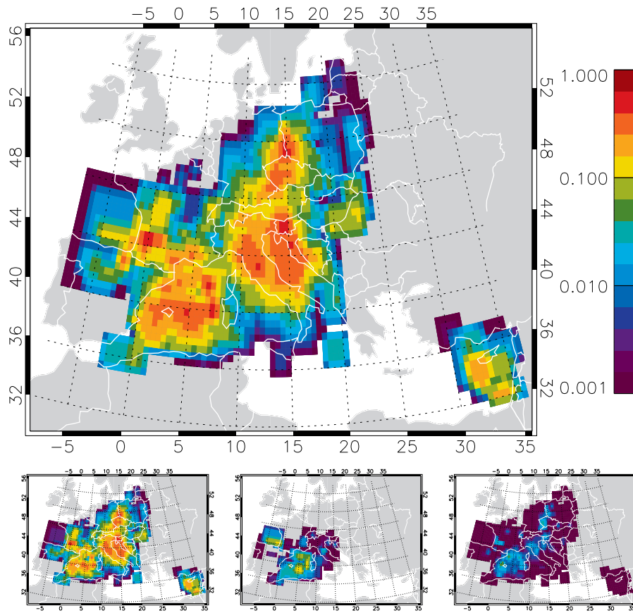
Fig. 2 Top: climatology of observed TLEs ( \text{TLEs} \cdot 10^{-3} \text{ km}^{-2} \text{ yr}^{-1} ) for 2009 to 2013. Bottom: climatology of observed sprites, elves and halos (left to right). All panels adopt the same color scale.
