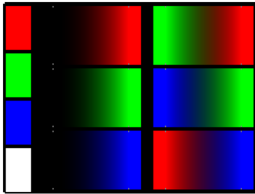
Fig. 9. Test image used for the calibration procedure. Left: pure red, green, blue, and white color patches. Middle: single color ramps. Right: dual color ramps as used in the patterns.
