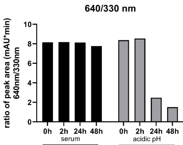
Supplementary Figure S4. Vem-L-Cy5 3 absorbance at 640 nm after long incubation in acidic medium.
