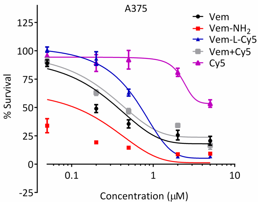
Supplementary Figure S6. Cy5 4 fluorophore does not contribute to Vem 1 cytotoxicity.
