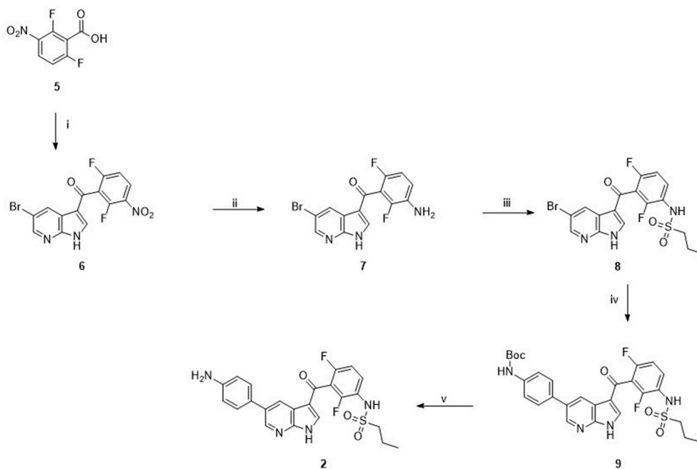
Scheme 1. Reagents and conditions: (i) a) dry DCM, dry DMF, oxalyl chloride, room temperature, overnight; b) \text{AlCl}_3 , 5-bromo-7-azaindole, DCE, 50 °C, overnight, 92%; (ii) conc. HCl, Fe, EtOH, THF, 75 °C, 3 h, 86%; (iii) dry DCM, 1-propanesulfonylchloride, pyridine, room temperature, overnight, 89%; (iv) MeCN, 4-( N -Boc-amino)phenylboronic acid, Pd(dppf) \text{Cl}_2 , 2 M \text{Na}_2\text{CO}_3 , MW, 160 °C, 30 min, 71%; (v) dry DCM, TFA, room temperature, 3 h, 98%.
