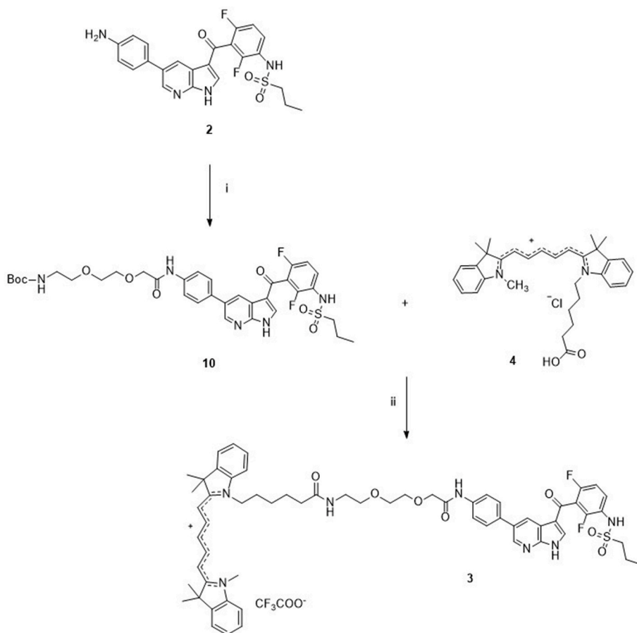
Scheme 2. Reagents and conditions: (i) dry DMF, 8-(Boc-amino)-3,6-dioxaoctanoic acid-DCA salt, HATU, DIPEA, room temperature, overnight, 81%; (ii) a) DCM, TFA, room temperature, 2 h, b) dry DMF, HBTU, DIPEA, room temperature, overnight, 49%.
