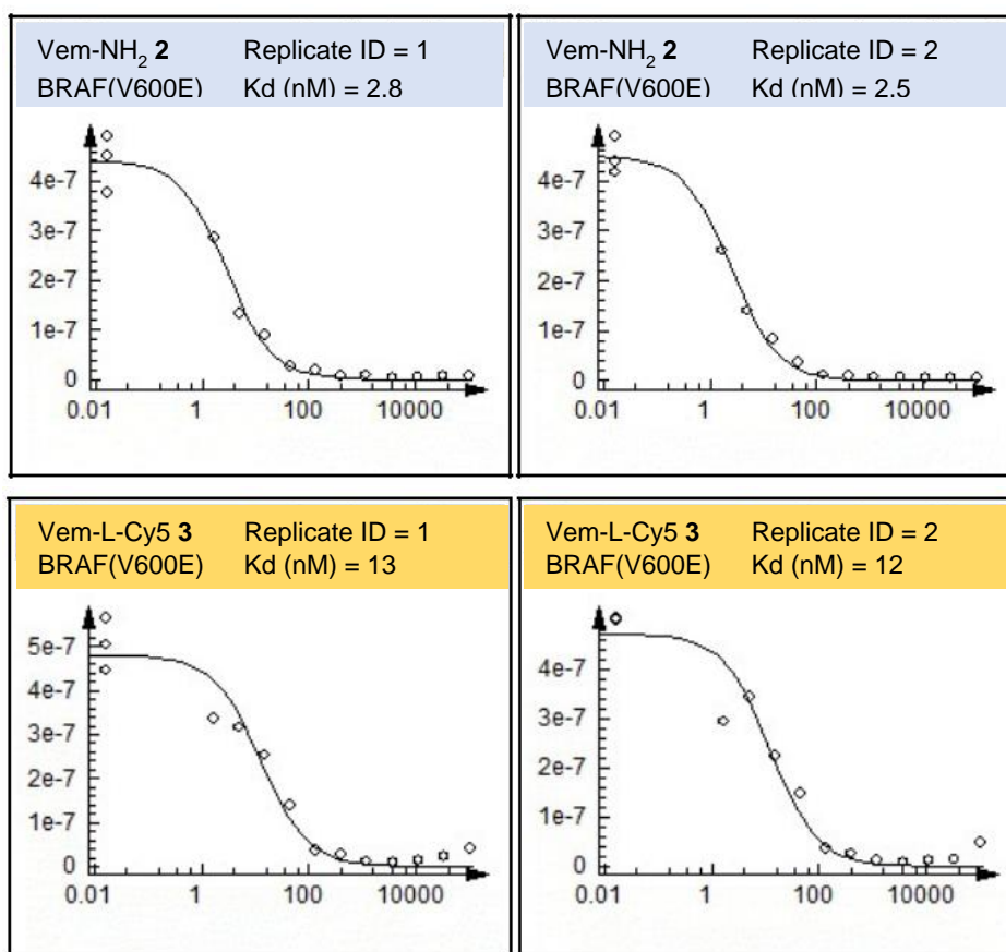
Supplementary Figure S5. Curve images for Vem-NH 2 2 and Vem-L-Cy5 3 .
