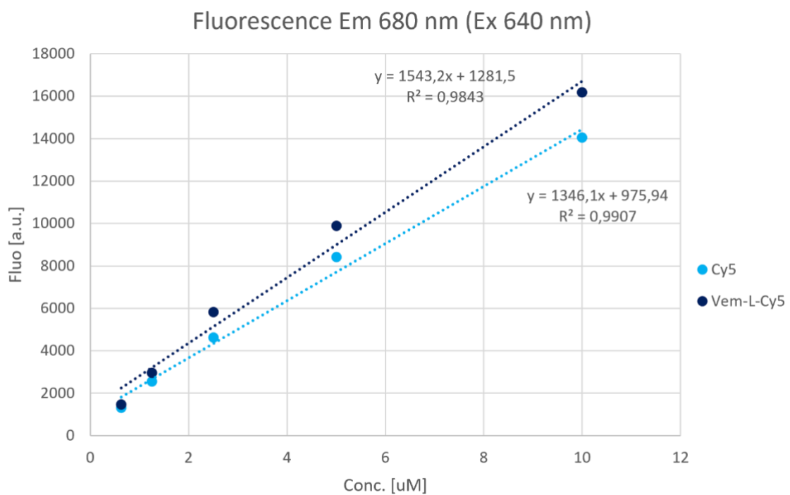
Supplementary Figure S2. Absorbance (upper) and fluorescence (lower) of Vem-L-Cy5 3 . Cy5 4 was used as standard. Em: emission; Ex: excitation
