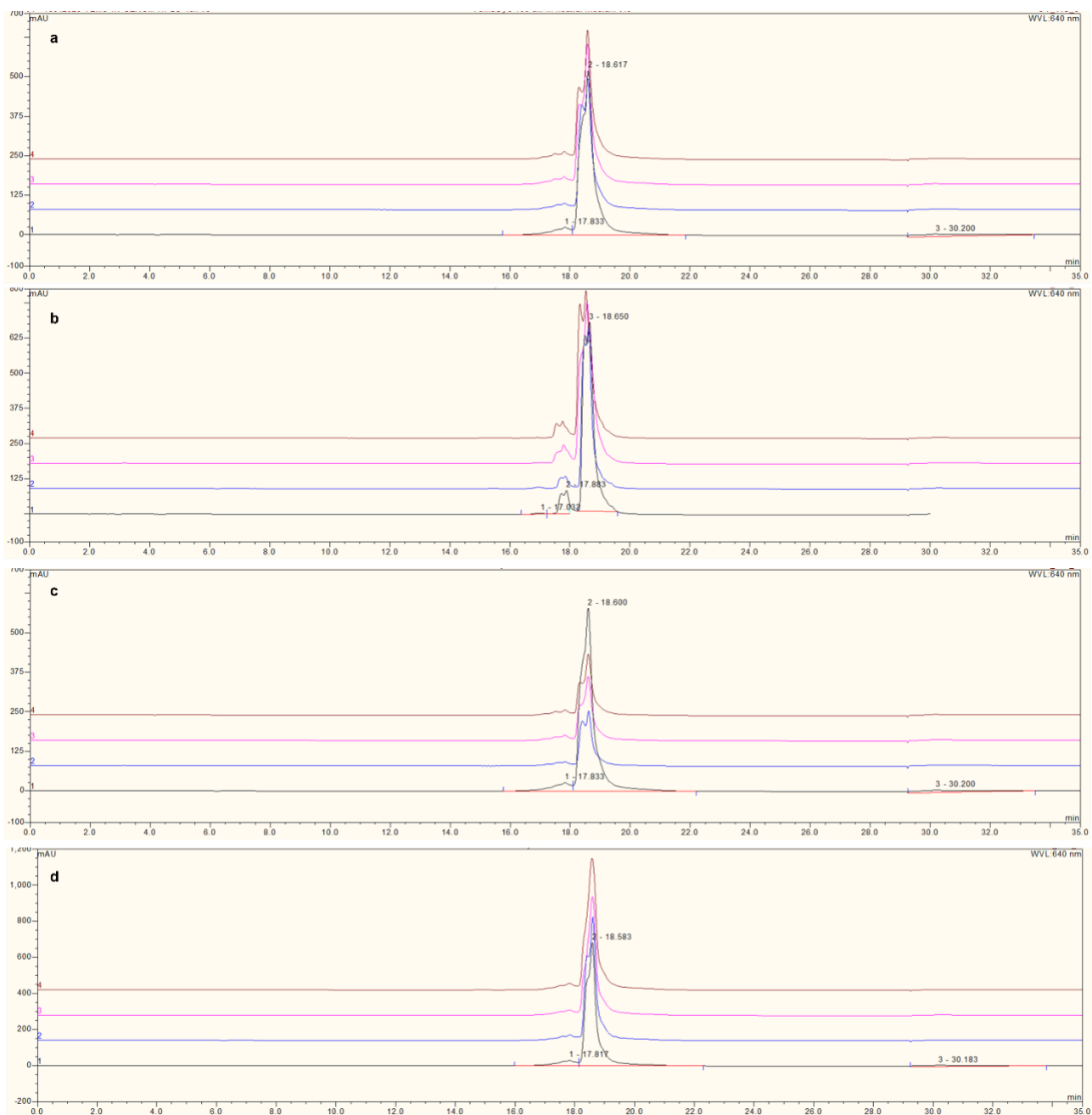
Supplementary Figure S3. Vem-L-Cy5 3 stability over time in different media and at different pH.
