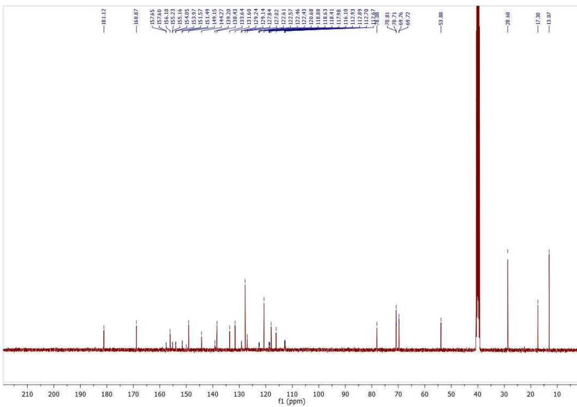
Supplementary Figure S7. 1 H NMR and 13 C NMR of compounds 2-10.
