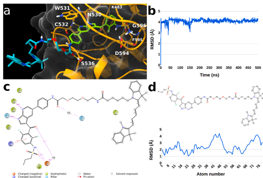
Fig. 5. Molecular modeling of Vem-L-Cy5 3 interaction with BRAF V600E .
