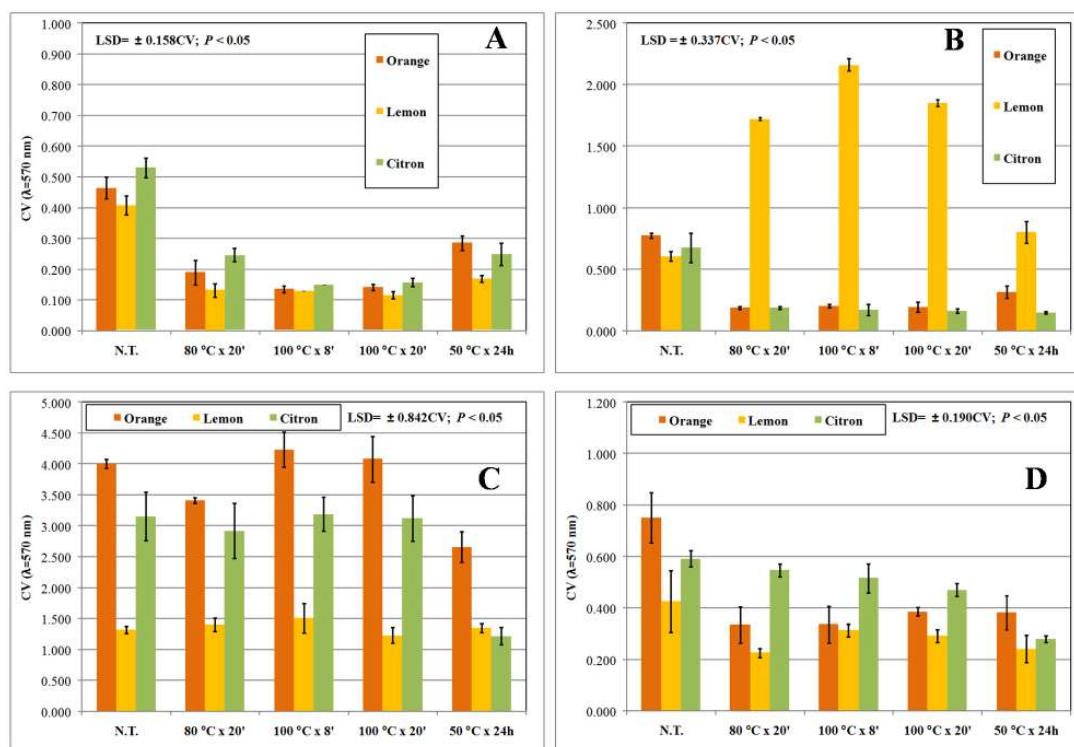
Figure 4. Biofilm biomass produced by S. caprae DSM 20608 (A), S. epidermidis UR63 (B), S. saprophyticus UR18 (C), and S. xylosoyus DSM 20266T (D) in the presence of different citrus peel water extracts. Mean values (bars \pm standard deviation) from the same strain were compared by Fisher's least significant difference (LSD) multiple-comparison test (95% Confidence Intervals); N.T.: not treated.
