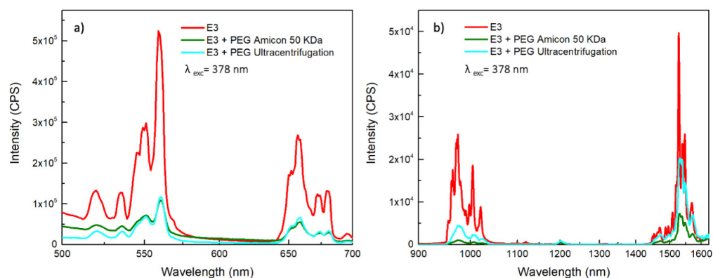
Figure 6. PL emission spectra in the visible (a) and IR (b) range of Er:Y 2 O 3 NPs sample E3 core and pegylated core/shell after purification ( \lambda_{\text{exc}} = 378 nm).
