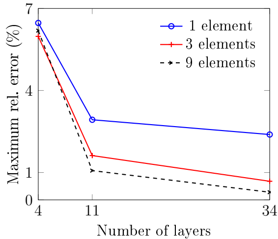
Figure 9: Difference between post-processed and analytical stress state. Different number of elements are used for the in-plane mesh, with S = 10 . The degree of the shape functions remains 4 in-plane and 3 through the thickness
