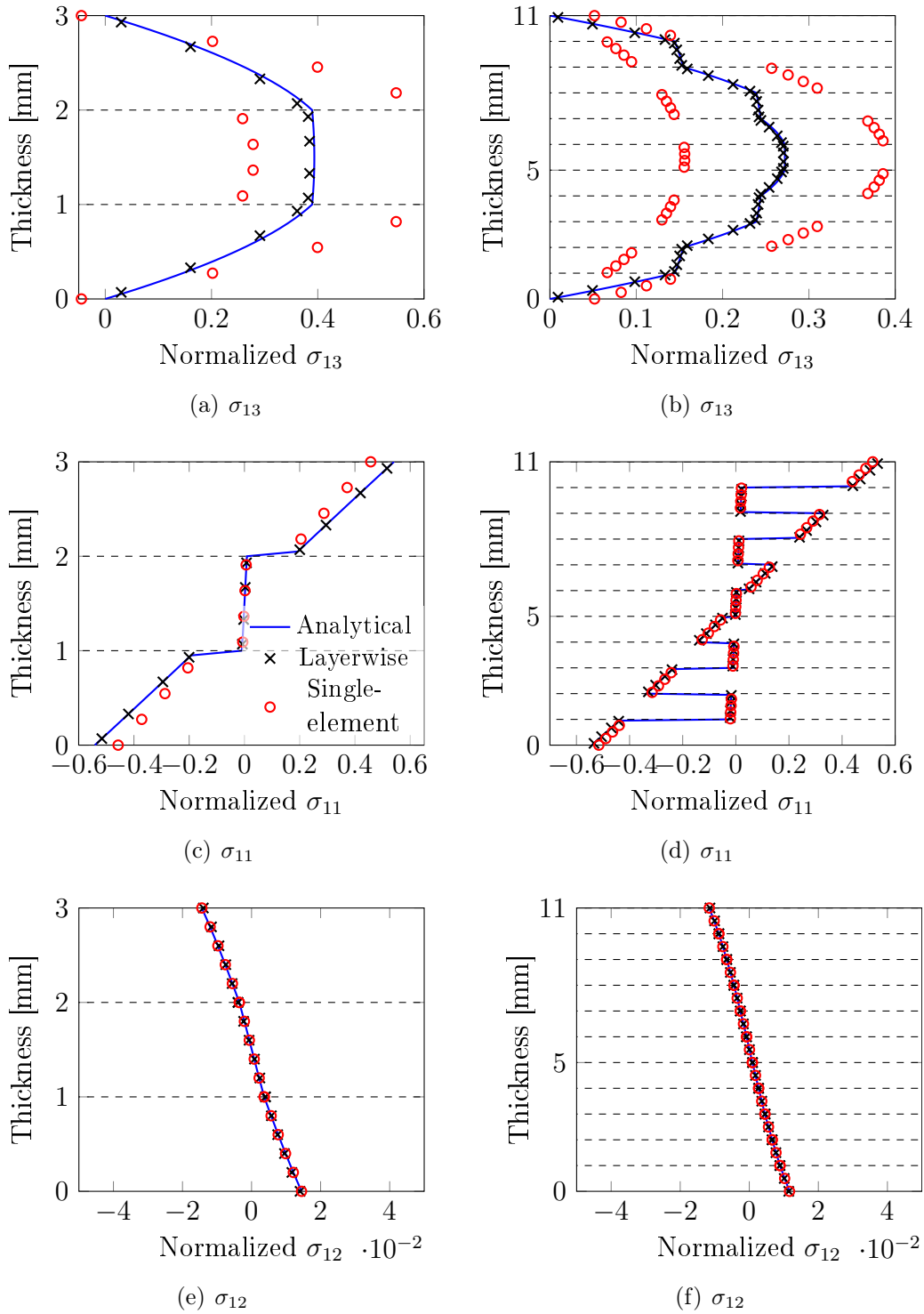
Figure 3: Computed solutions for the 3D Pagano plate problem with 3 and 11 layers at the position X = 0.25L and Y = 0.25L . The blue solid line represents the analytical solution, the black cross represent the solution using the layerwise approach, and the red circles represent the solution using the single element approach (without post-processing)
