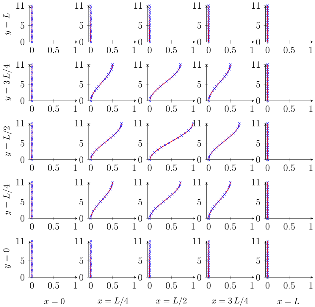
Figure 7: Recovered (red solid line) \sigma_{33} compared to the analytical one (blue crosses) for several in plane positions. L is the total length of the plate, that in this case is L = 110 mm (being L = St with t = 11 mm and S = 10 ), while the number of layers is 11.
