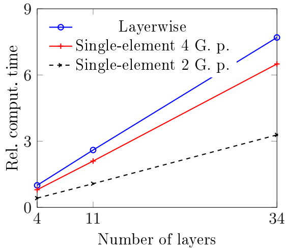
Figure 4: Relative computational time with respect to the number of layers. The single-element approach (red and black lines, using 4 and 2 integration points per layer respectively) is less time consuming than the simulation with one element per layer (blue line). In this case, there are 9 quartic elements along each in-plane direction and cubic shape functions through the thickness, corresponding to 1,183, 5,746 and 17,407 degrees of freedom for the layerwise approach, and 676 for the single-element approach
