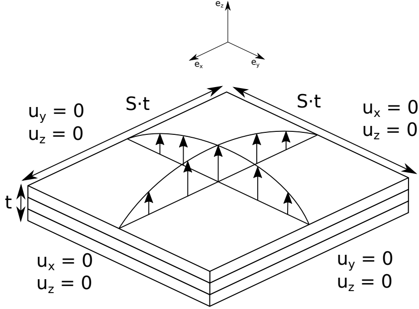
Figure 2: 3D problem used as a test case, proposed by Pagano [28]
