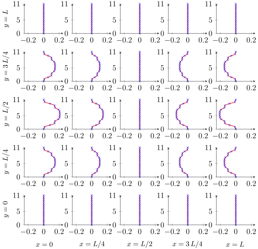
Figure 5: Recovered (red solid line) \sigma_{13} compared to the analytical one (blue crosses) for several in plane positions. L is the total length of the plate, that in this case is L = 110 mm (being L = St with t = 11 mm and S = 10 ), while the number of layers is 11.
