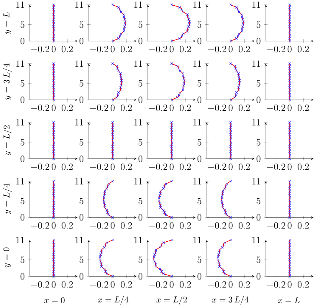
Figure 6: Recovered (red solid line) \sigma_{23} compared to the analytical one (blue crosses) for several in plane positions. L is the total length of the plate, that in this case is L = 110 mm (being L = St with t = 11 mm and S = 10 ), while the number of layers is 11.
