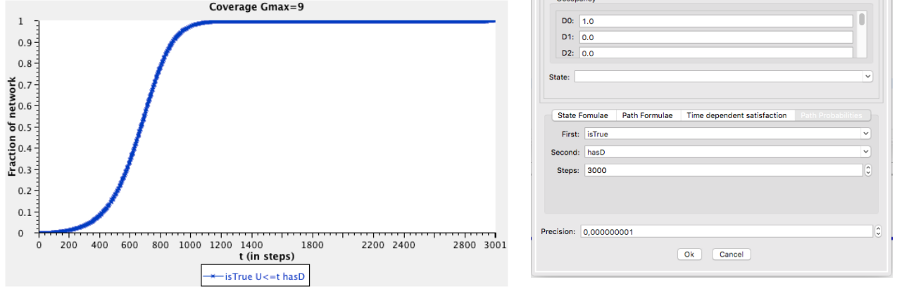
Figure 7: Network coverage for a model with G_{max} = 9 , N = 2500 , n = 500 , s = 100 and c = 50 .
