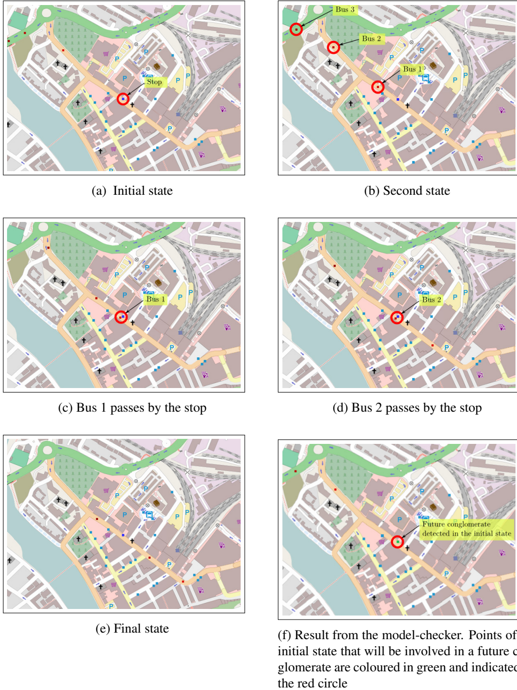
Figure 26: Spatio-temporal conglomerate.
