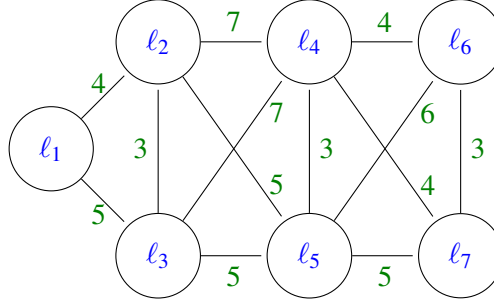
Figure 8: Representation of the space of the epidemic model. The nodes \ell_1, \dots, \ell_7 represent the different communities; the edges represent the link between the communities through the water basin. The green numbers correspond to the values w of the weight function for each edge.
