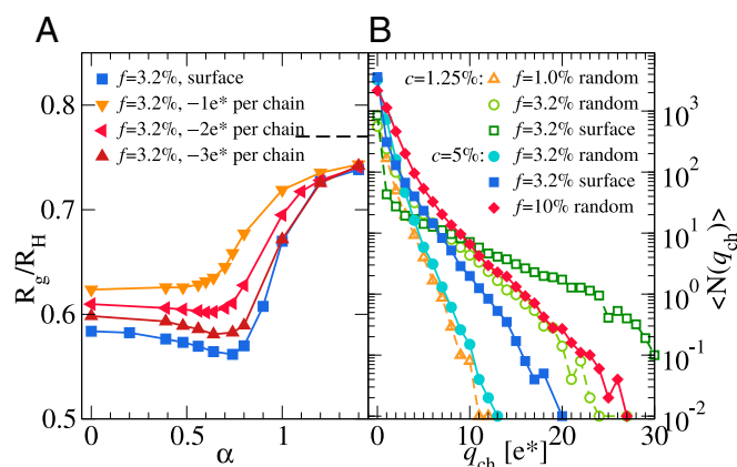
Fig. 5. Ratio R_g/R_H for c = 5\% surface-charged microgels (A) and distribution N(q_{ch}) of number of charges per chain. The dashed line indicates the HS value. (B) Surface-charged microgels are shown with filled symbols, while open triangles indicate microgels with f = 3.2\% for which charges are constrained to be found as one, two, or three charges on each external chain, indicated as -1e^* , -2e^* , -3e^* per chain, respectively.
