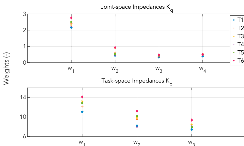
Figure 8. Square root of the sum of the squared weight values of the joint-space and task-space impedances T1 to T6 denote target 1 to target 6, respectively.
