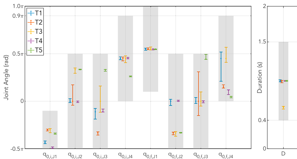
Figure 7. Sensitivity of task performance to the movement parameters for targets 1 to 5 Gray bars depict the upper and lower bounds of the search space of the DIRECT-L optimization algorithm. The upper (respectively lower) error bar depicts the upper (respectively lower) value of the error to miss the target. Dots within the error bar depict the optimal movement value (Table 1). T1 to T5 denote target 1 to target 5, respectively.
