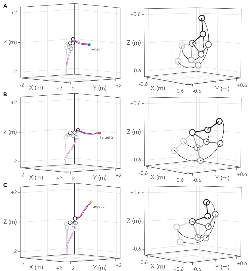
Figure 3. Simulation results for targets 1, 2, and 3, shown in panels A, B, and C, respectively (Left column) Time-sequence of upper-limb and whip model. Three frames of the simulation were taken: at the start of the movement, at the moment when the whip hit the target, and a moment between the two. Black circles depict the shoulder, elbow and hand of the upper-limb model. Purple circles depict the point-masses of the whip model. Opacity of the color increases from the start to the end of the movement. (Right Column) Time-sequence of the corresponding optimal trajectories of elbow and end-effector. Four frames are plotted from the start to the end of the movement, i.e., for time 0 \leq t \leq D , where D is the duration of the virtual (zero-torque) trajectory (Equation 3).
