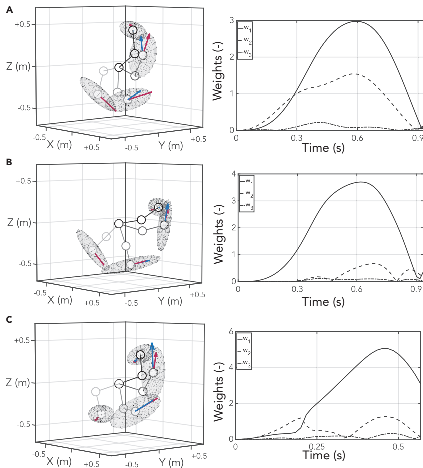
Figure 9. Task-space stiffness ellipsoids for targets 1, 2, and 3, shown in panels A, B, and C, respectively
