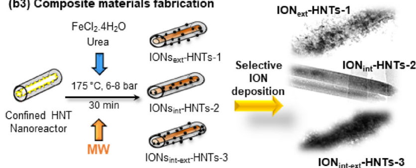
Fig. 4. (a) MW-assisted high-pressure reactor for solvothermal processes. (b) Application of MW-assisted high-pressure to: (b1) hydrothermal heterogeneous catalytic decomposition of microcrystalline cellulose using zeolite beta (b2) Solvothermal syntheses of iron oxide nanoparticles, (b3) Solvothermal syntheses of composite materials.
