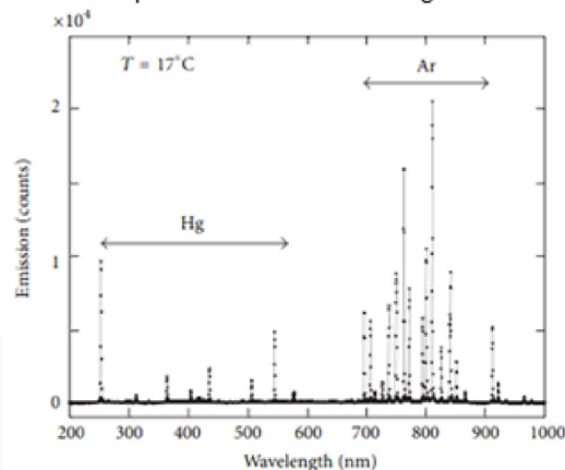
The emission spectrum of the integrated MW/UV lamp in the 200 ÷ 1000 nm region
