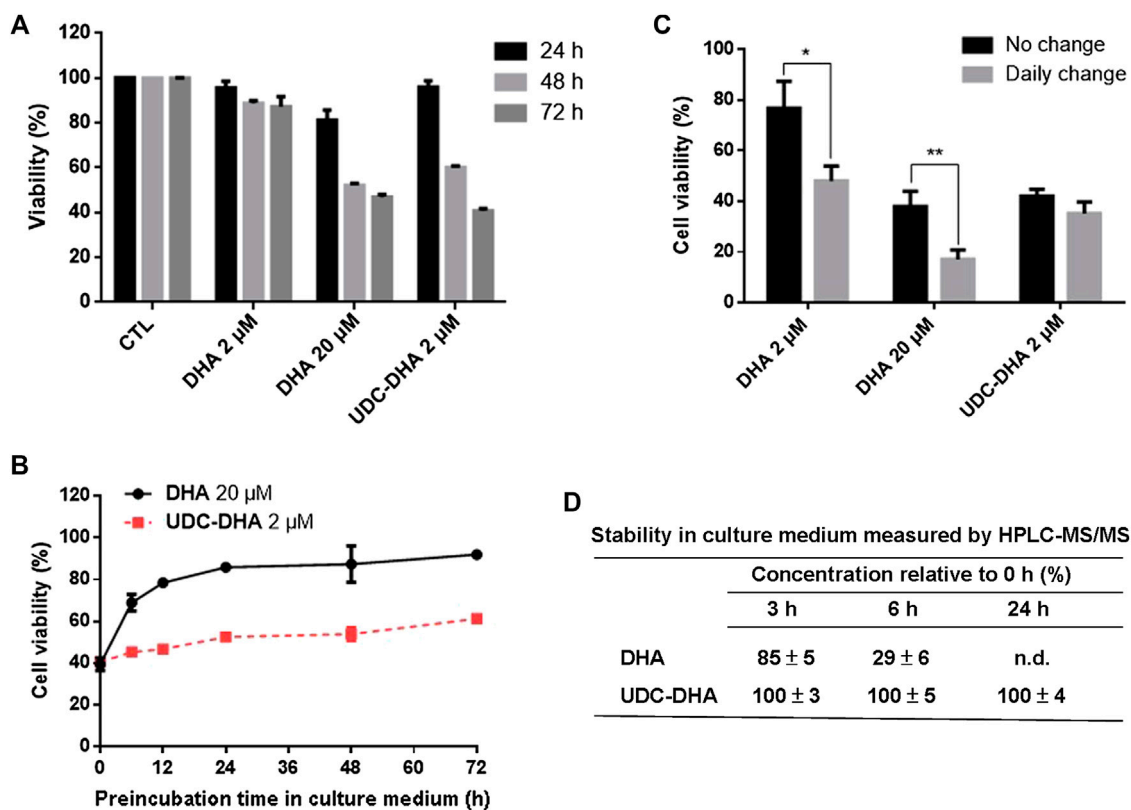
FIGURE 6 | UDC-DHA is more stable than DHA. (A) Time course of the effect of DHA and UDC-DHA on cell viability revealed that UDC-DHA acted gradually and more persistently than DHA. (B) Pre-incubation of DHA but not UDC-DHA in culture medium greatly reduced growth inhibitory effect. DHA and UDC-DHA were incubated in culture medium at 37°C for various time periods and then added to HepG2 cells for 72 h, followed by the MTT assay. Results were obtained from at least three independent experiments and data are presented as mean \pm SEM. (C) Daily change of culture medium containing DHA but not UDC-DHA significantly increased the growth inhibitory effect. HepG2 cells were treated with indicated concentrations of DHA or UDC-DHA for 72 h with or without daily change of drug containing medium and then subjected to the MTT assay. Results are presented as mean \pm SEM of three independent experiments. *, p < 0.05 ; **, p < 0.01 . (D) Stability of DHA and UDC-DHA in cell culture medium measured by HPLC-MS/MS. DHA (20 \mu M) or UDC-DHA (2 \mu M) was incubated in cell culture medium and 500 \mu l aliquots were extracted with ethyl acetate for HPLC-MS/MS analysis. The concentrations of DHA and UDC-DHA at 3, 6 or 24 h were calculated by comparison with that of the 0 h. The data are presented as mean \pm SEM of three experiments. n.d., not detected.
