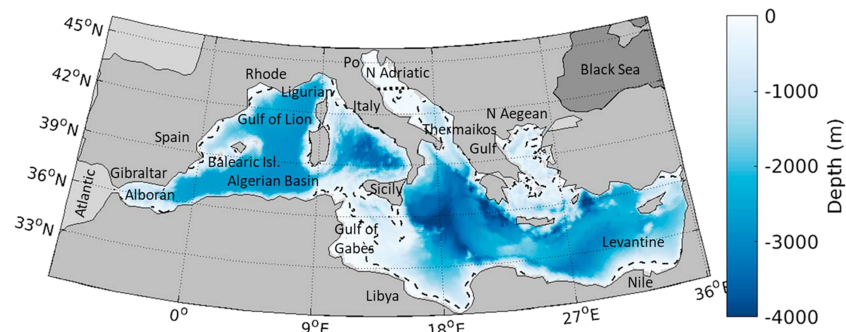
Figure 1. Domain and bathymetry of the Mediterranean Sea model. The western boundary of the model extends into the Atlantic as a buffer area, but results will be only shown for the Mediterranean area in the map, that is, from 5°W. The dashed line represents the 200-m isobaths; the dotted line represents latitude 43.5°N, here delimiting the North Adriatic.
