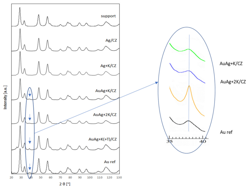
Figure 2. XRD results: diffraction patterns of the catalysts.
