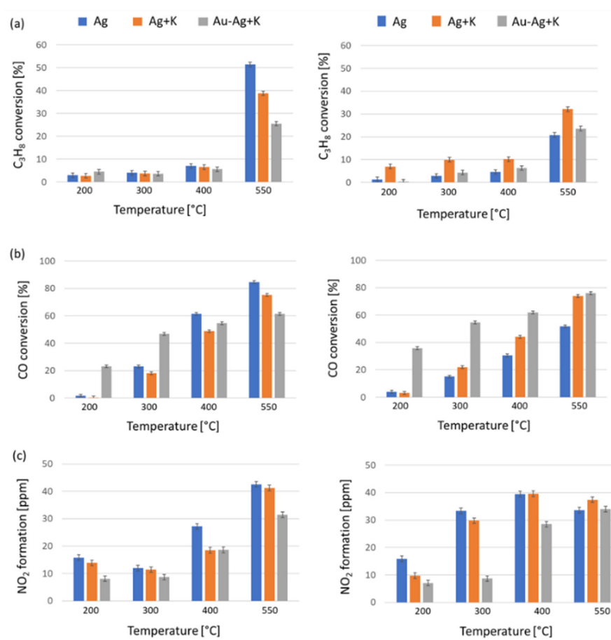
Figure 8. Activity results for Ag/CZ, Ag+K/CZ, and AuAg+K/CZ in complex stream: (a) C 3 H 8 combustion, (b) CO oxidation, and (c) NO 2 formation without (left) and with water vapor (right) in the inlet stream.
