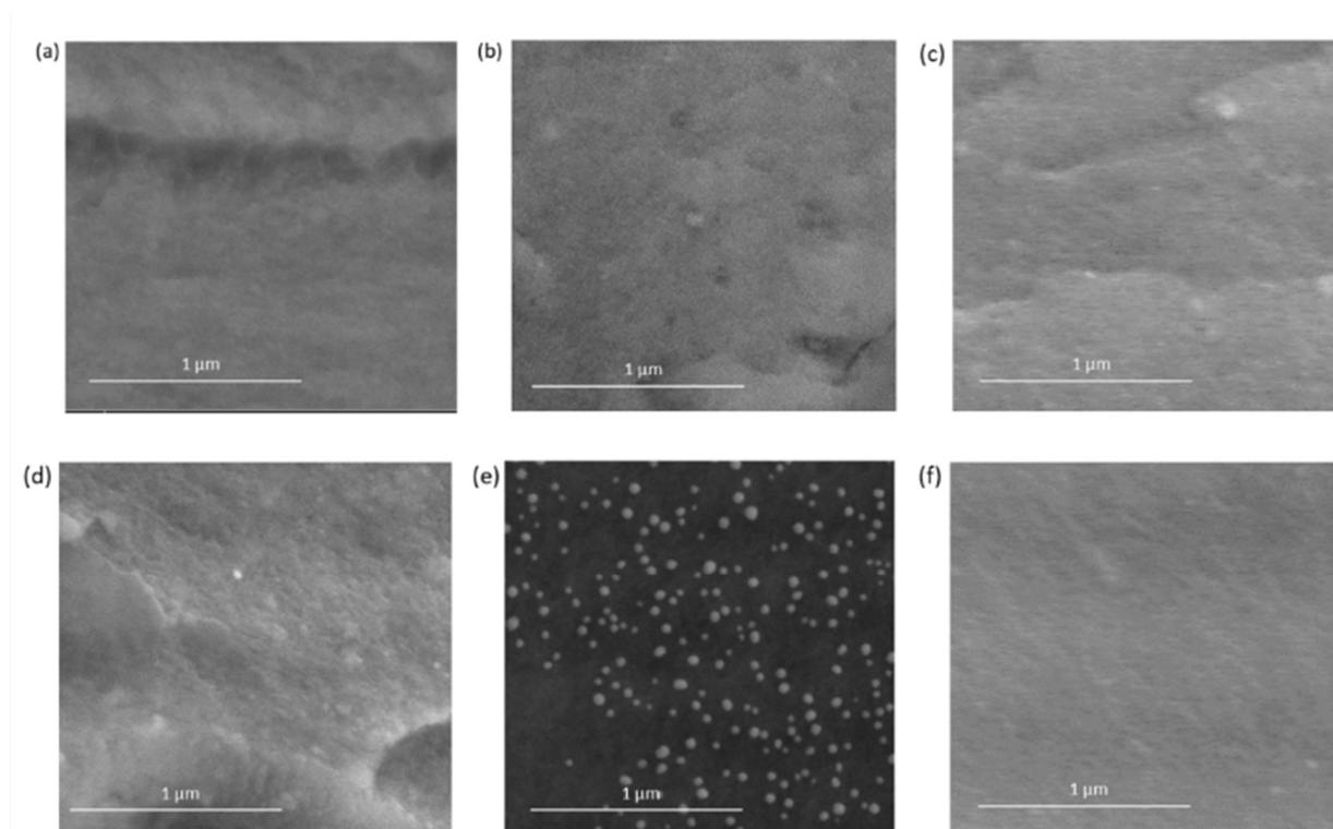
Figure 1. SEM images of silver catalysts: (a) Ag/CZ, (b) Ag+K/CZ, and the bimetallic systems: (c) AuAg+K/CZ, (d) AuAg+2K/CZ, (e) AuAg+K(+T)/CZ, (f) Au reference at the magnification of 100 000 times.
