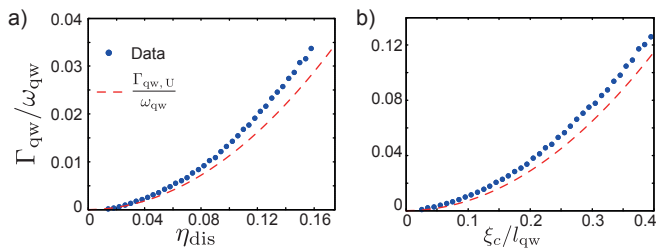
FIG. 4. a) Plot of the FWHM \Gamma_{\text{qw}} of the ISB optical density \rho_{\text{qw}} as a function of the disorder strength \eta_{\text{dis}} (blue solid dots). b) Plot of \Gamma_{\text{qw}} as a function of the disorder correlation strength \xi_c . Disorder parameters: \xi_c/l_{\text{qw}} = 0.5 (in panel a), \eta_{\text{dis}} = 0.4 (in panel b). Fermi energy E_F/\hbar\omega_{\text{qw}} \approx 0.5 . In both panels, the red dashed line is the Unuma-linewidth given by Eq. (23). To numerically implement Eq.(15) we used a finite-width delta function, with small linewidth \gamma_\delta/\omega_{\text{qw}} \approx 0.002 , which is then subtracted from the numerical data.
