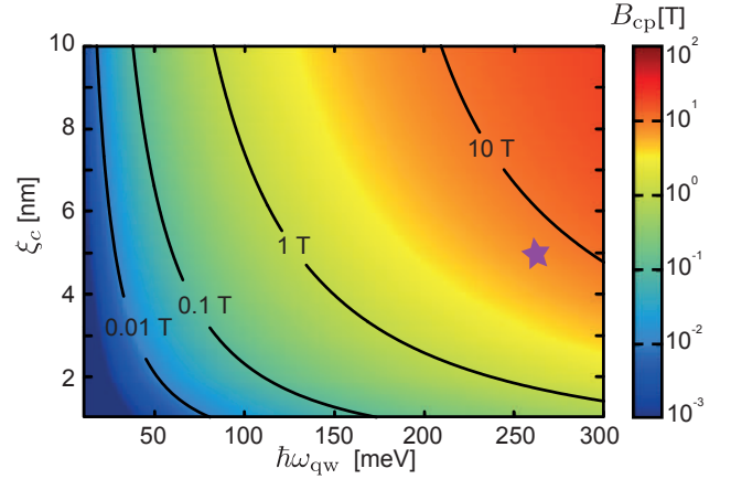
FIG. 11. Log-scale contour-plot of the cavity-protection magnetic field B_{cp} as defined in (37) as a function of the intersubband frequency \omega_{q\dot{w}} and the disorder correlation length \xi_c . Here, B_{cp} is given in units of Tesla, \hbar\omega_{q\dot{w}} is given in meV, and \xi_c in nm. The disorder amplitude is kept constant to \xi_0 = 0.3 nm. The effective Bohr magneton corresponding to the effective mass of electrons in GaAs is used, \mu_B^* \approx 0.86 meV / T. The purple star indicates the position of the setup inspired by [18] described in the text.
