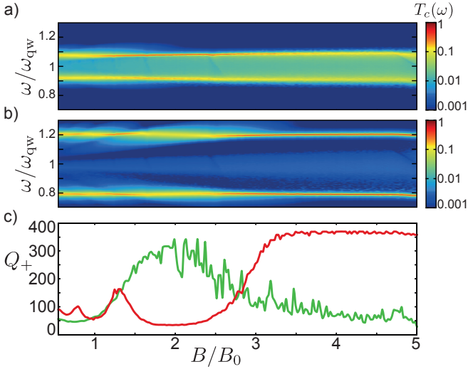
FIG. 10. a-b) Logscale color plot of the cavity transmission T_c(\omega) as a function of the magnetic field B/B_0 and the external incident frequency \omega/\omega_{q\dot{w}} . In a) \Omega_R/\omega_{q\dot{w}} = 0.15 , in b) \Omega_R/\omega_{q\dot{w}} = 0.4 . c) Quality factor of the upper polariton as a function of the magnetic field B/B_0 . The green and red solid lines refer to the \Omega/\omega_{q\dot{w}} = 0.15 and 0.4 values used in panel a) and b), respectively. Parameters for all plots: \omega_c = \omega_{q\dot{w}} , \eta_{\text{dis}} = 0.1 , \xi_c/l_{q\dot{w}} = 1 , Fermi energy E_F/\hbar\omega_{q\dot{w}} = 0.5 . For these parameters, the ISB quality factor (without cavity) is found to be Q_{q\dot{w}} \approx 22 , while the cavity quality factor is set to the realistic value Q_c = 200 .
