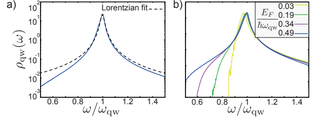
FIG. 3. a) Optical density \rho_{\text{qw}}(\omega) (blue solid line) and Lorentzian fit (black dashed line). b) Optical density \rho_{\text{qw}}(\omega) calculated for increasing values of the Fermi energy E_F . Disorder parameters: \eta_{\text{dis}} \approx 0.06 , \xi_c/l_{\text{qw}} = \sqrt{2} . In a) the Fermi energy is fixed to E_F/\hbar\omega_{\text{qw}} \approx 0.6 , while in b) a range of values is used as indicated in the legend.
