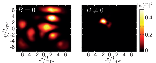
FIG. 7. Illustrative examples of the real-space wavefunction of a n = 1 subband eigenstate in the presence of disorder in the B = 0 (left) and B/B_0 = 0.5 (right) cases. These eigenstates are obtained via exact diagonalisation, as detailed in App. C, of a square system with lateral size L_{x,y}/l_{qw} = 14 . Other parameters: E_F/(\hbar\omega_{qw}) = 0.5 , \eta_{dis} \approx 0.03 , \xi_c/l_{qw} \approx 4 .
