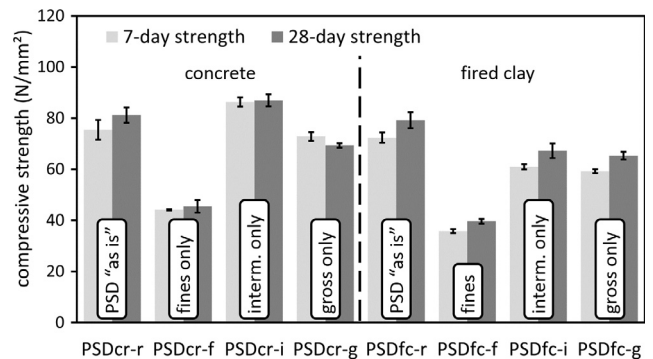
Fig. 7. Effects of Particle Size Distribution of aggregates on compressive strength.
