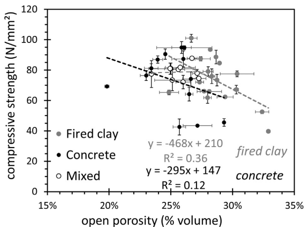
Fig. 12. Compressive strength plotted versus the open porosity (trends are qualitative).
