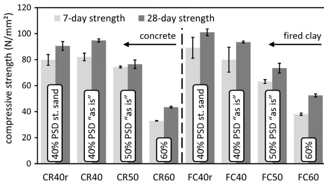
Fig. 6. Results for aggregate content increasing from 40% to 60%.
