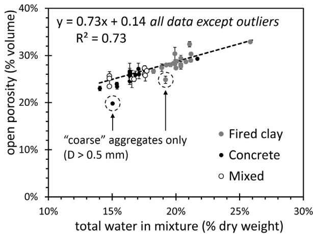
Fig. 11. Relation between open porosity and water added to the fresh mixture.
