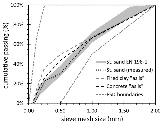
Fig. 2. Adopted Particle Size Distributions (PSDs).
