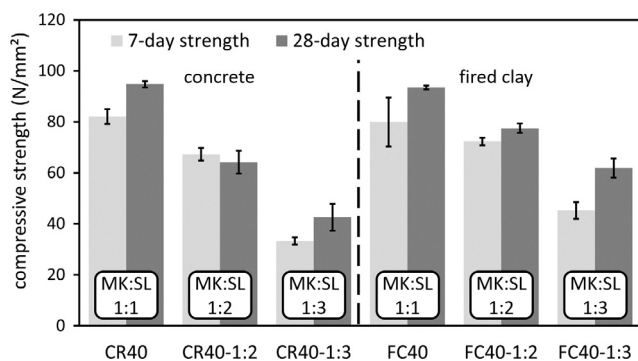
Fig. 8. Results for various Metakaolin:Slag (MK:SL) ratios.
