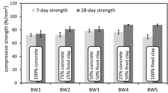
Fig. 4. Results of mixtures with blended aggregate types (40% dry weight of aggregate content).
