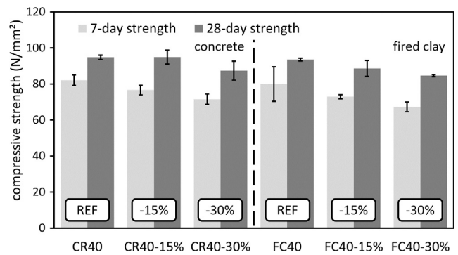
Fig. 9. Effect of K-silicate base reduction on compressive strength.
