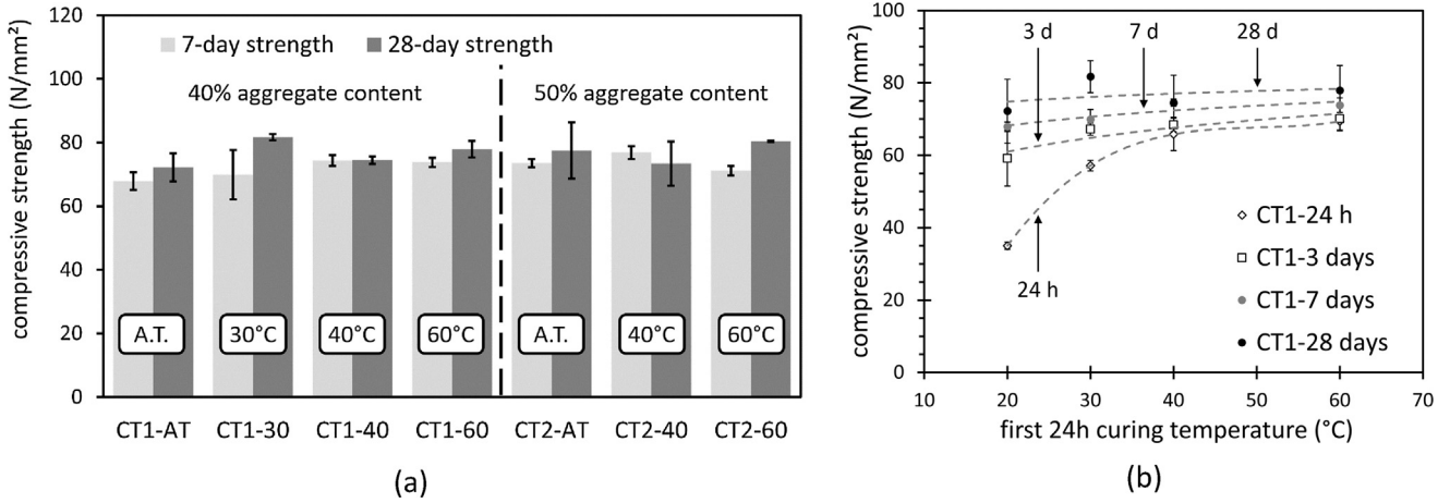
Fig. 5. Effect of curing temperature during the first 24 h: (a) comparison of results, and (b) evolution of strength.
