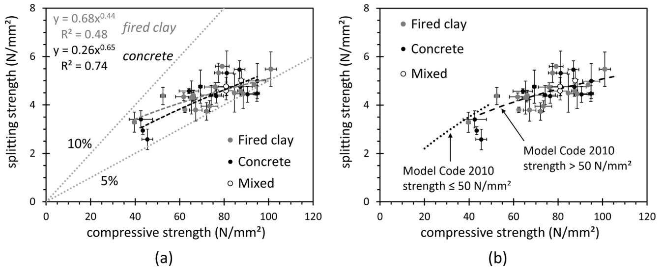
Fig. 15. Splitting vs. compressive strength measured at 28 days.
