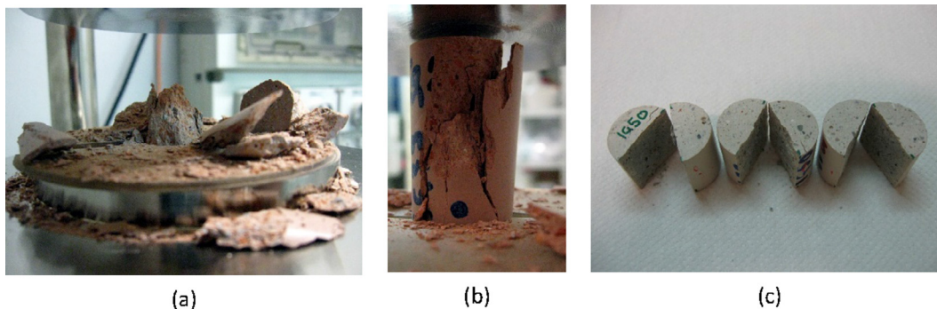
Fig. 3. Typical failure modes in compression: (a) explosive, with disintegration of the sample, (b) less sudden; and (c) typical failures in splitting along the loaded diametral plane.
