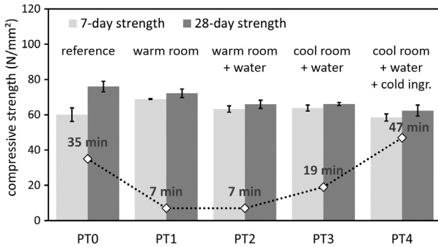
Fig. 10. Strength and open time for different conditions during preparation.
