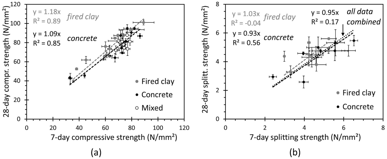
Fig. 14. Values measured at 7 and 28 days for: (a) compressive strength, and (b) splitting strength.
