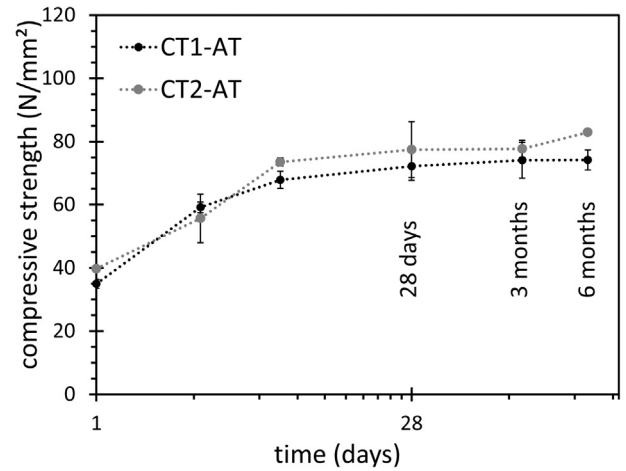
Fig. 13. Evolution of compressive strength over 6 months for mixtures CT1-AT and CT2-AT.
