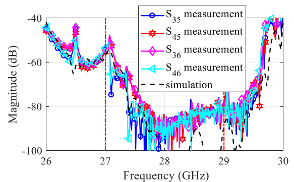
FIGURE 11. Measured and simulated Ka-band transmission coefficients between the WR42 and WR28 waveguide ports of the K/Ka-band feeding network. The simulated data refer to the de-embedded CAD model described in the text.
