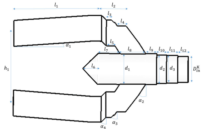
FIGURE 4. Section view of the K-band ortho-mode junction OMJ #1.
