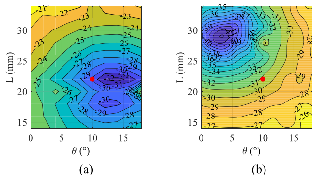
FIGURE 13. Contour maps of the simulated performance of the K/Ka-band feeding network as a function of the length L and rotation angle \theta of an elliptical-waveguide line connected to its circular waveguide port. The major and minor axes of the elliptical waveguide are d_x = 12.440 mm and d_y = 12.040 mm, respectively. The red dot refers to the manufactured elliptical waveguide line. (a) Maximum cross-polar transmission coefficient in K band. (b) Maximum cross-polar transmission coefficient in Ka band.
