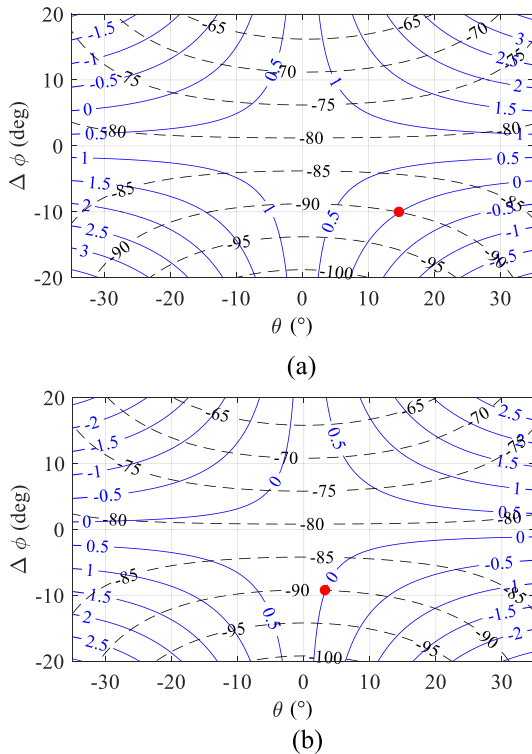
FIGURE 12. Amplitude (blue solid lines) (dB) and phase (black dashed lines) (deg) contour plots of the linear-transmission-coefficients ratio of the prototype cascaded with an ideal rotated elliptical-waveguide line. The red dots denote the elliptical-waveguide parameters for single-band compensation (reported in the text). (a) S_{V,3}/S_{H,3} (K band). (b) S_{V,5}/S_{H,5} (Ka band).
