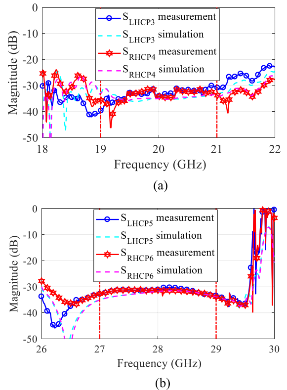
FIGURE 14. Measured and simulated cross-polar transmission coefficients of the K/Ka-band feeding network cascaded with the compensation elliptical waveguide at the circular-waveguide port. (a) Cross-polar transmission coefficients in K band from the WR42 ports 3 and 4 to the uncoupled circular polarizations at the circular waveguide port. (b) Cross-polar transmission coefficients in Ka band from the WR28 ports 5 and 6 to the uncoupled circular polarizations at the circular waveguide port.
