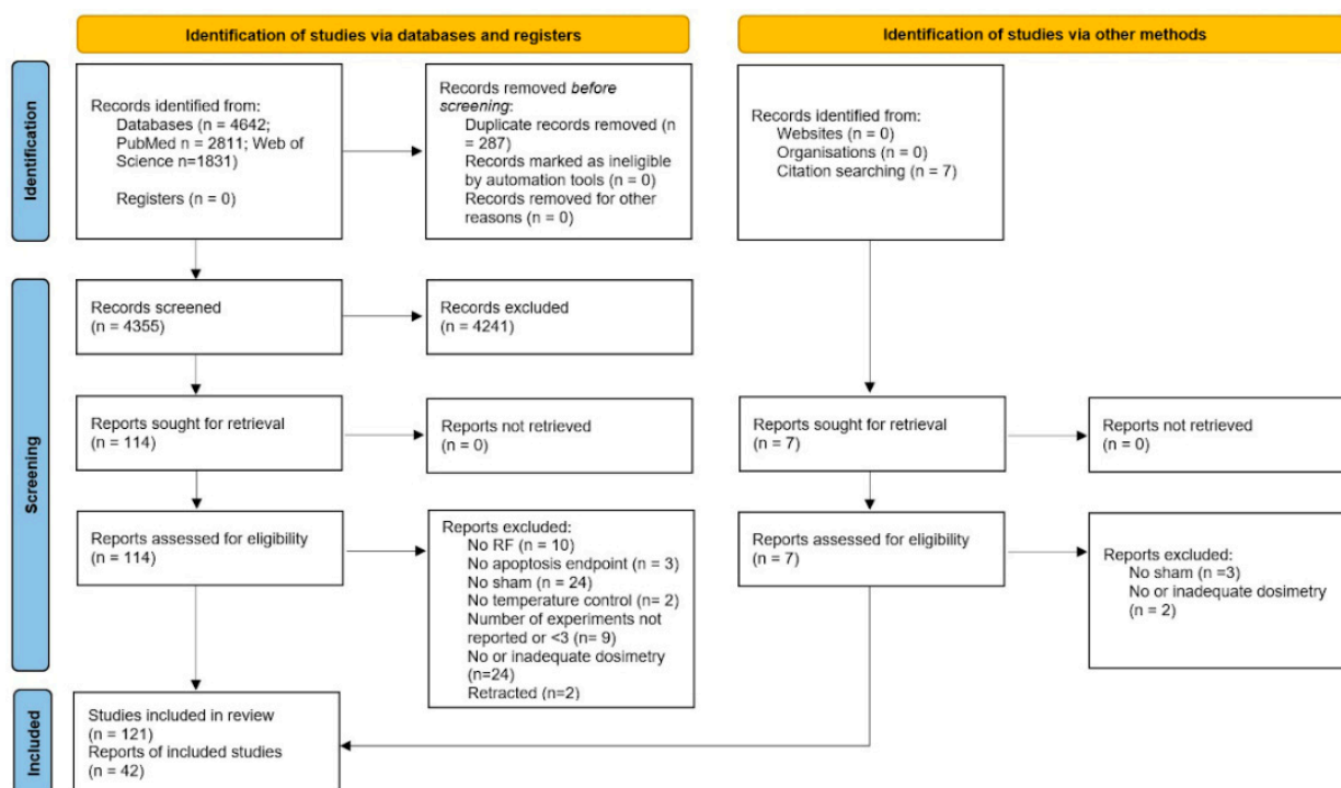
Figure 1. PRISMA flowchart.
