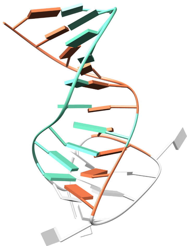
Figure 4. Ribbon representation of RE31 highlighting the continuous stacking of bases from the duplex to the quadruplex region.
