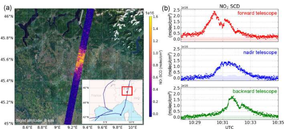
Figure 18. HAIDI measurement at 8 km altitude of the Milan outflow during E-EU-09: (a) pixel-resolved NO 2 slant column densities observed by the nadir camera (marked by the red square on the map). The grey arrow indicates the direction of the flight. An enhancement of up to 1.5 \times 10^{16} molec cm -2 over the background is observed northeast of Milan (red-coloured circle), (b) NO 2 slant column densities averaged over the whole swath for all three telescopes: forward (top) nadir (middle) and backward (bottom). The height of the plume centre is estimated from the time difference of the maxima. Sources of background imagery: ESRI, DigitalGlobe, GeoEye, i-cubed, USDAFSA, USGS, AEX, Getmapping, Aerogrid, IGN, IGP, swisstopo, and the GIS User Community.
