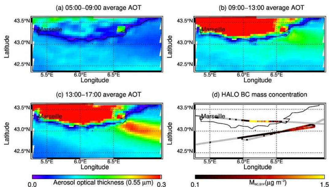
Figure 31. (a–c) Aerosol optical thickness at 0.55 μm as retrieved from SEVIRI from 05:00 to 17:00 UTC on 24 July 2017. (d) E-EU-07 flight track, colour coded with BC mass concentration ( M_{BC} ). For better contrast, the scale for M_{BC} ranges from 0.1 to 1.5 μg m -3 . Grey colour on the flight track indicates values below 0.1 μg m -3 . The mass concentration reached values up to 7 μg m -3 at the French coast.
