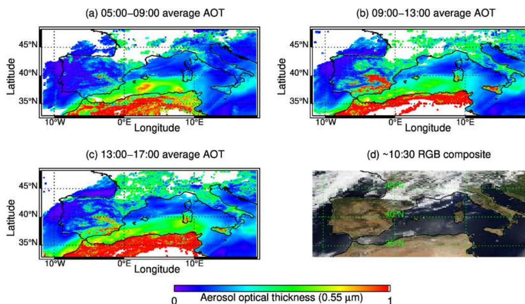
Figure 32. (a–c) Aerosol optical thickness at 0.55 μm as retrieved from SEVIRI from 05:00 to 17:00 UTC on 11 July 2017, (d) MODIS RGB composite figure showing corrected reflectance at 10:30 UTC ( https://worldview.earthdata.nasa.gov/ , last access: 21 March 2022). The MODIS RGB composite is created combining red, green, and blue bands into one picture. White areas are clouds. The E-EU-03 flight track (in red) is superimposed in panel (d).
