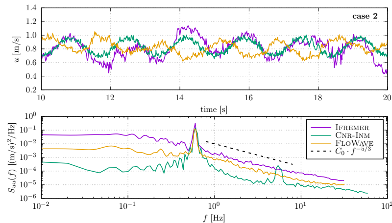
Figure 6. Time histories (top) of the ADV streamwise velocity u measured at the top-dead centre of the rotor for case 2 and their corresponding PSD (bottom) at IFREMER, FLOWAVE and CNR-INM. The PSD panel also includes Kolmogorov’s -5/3 power law.
