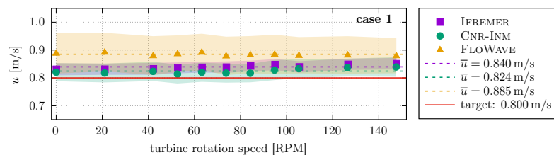
Figure 7. Time average (markers) and standard deviation (shading) of the ADV stream-wise velocity u versus turbine rotational speed for current-only case 1 at all facilities. Dashed lines are the average of u for case 1 at all rotational speed settings per facility; the red line is the target value of 0.8 m/s.
