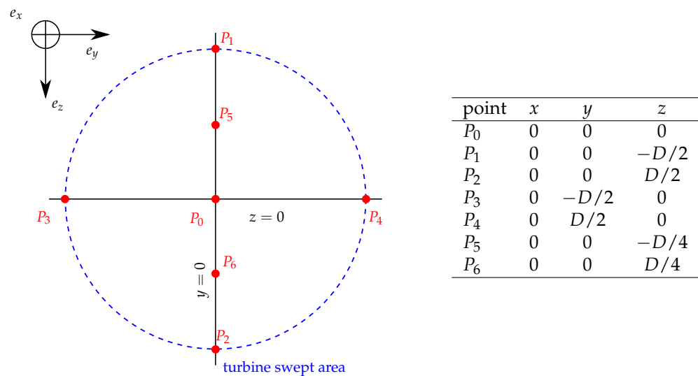
Figure 4. Front view of the ADV measurement points describing the swept area of the turbine and their coordinates expressed in diameter D = 0.724 m. Points 0 to 2 and 5 and 6 are acquired at IFREMER. Points 0 to 2 are acquired at CNR-INM. Points 0 to 4 are acquired at FLOWAVE.
