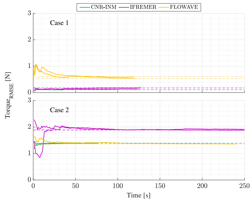
Figure 18. Stabilisation of the torque RMSE at TSR = 4 for case 1 (top) and 2 (bottom) at all facilities. Dashed lines are the RMSE value of the whole time series; same-colour curves are repeat tests when available.
