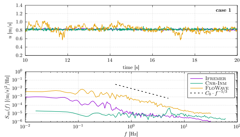
Figure 5. Time histories (top) of the ADV streamwise velocity u measured at the top-dead centre of the rotor for case 1 and their corresponding PSD (bottom) at IFREMER, FLOWAVE and CNR-INM. The PSD panel also includes Kolmogorov’s -5/3 power law.
