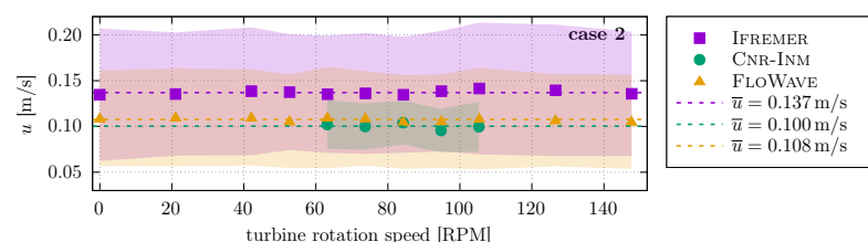
Figure 10. Variation of the time-averaged (markers) and standard deviation (shading) of the horizontal wave orbital velocity u with rotational speed for case 2 at all facilities, obtained with the ADV. Dashed lines are the average of horizontal wave orbital for case 2 at all rotational speed settings per facility.
