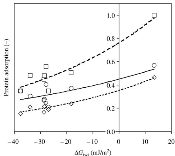
Figure 6 Correlation between protein adsorption at the concentration of 3 mg/ml and free energy of interfacial interaction ( \Delta G_{iwi} ). (□) Albumin; (○) fibrinogen; (◇) IgG. Interpolation of experimental data is reported as line. Data were normalized with respect to the value of albumin adsorbed on CA membrane.
