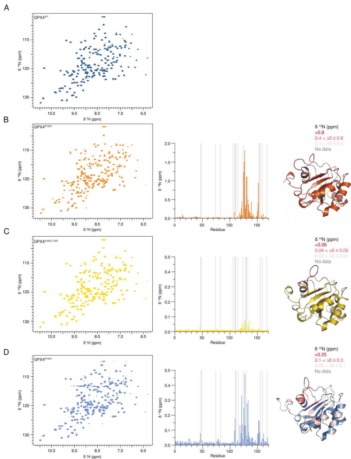
Figure S4. 1 H- 15 N HSQC spectra for WT and mutant GPX4 indicate all proteins are well folded, related to Figures 2 and 3 . 1 H- 15 N HSQC spectra are shown for (A) GPX4 WT , (B) GPX4 R152H , (C) GPX4 I129S;L130S , and (D) GPX4 R152K (left). Chemical shift perturbation (CSP) plots, \Delta\delta , for backbone amide residues are shown relative to GPX4 WT , indicating that most CSPs map to the polypeptide backbone of the fin-loop region (middle). Gray bars indicate unassigned residues. CSPs are mapped onto the crystal structures of the respective mutants (right). PDB: 2OBI is used for the GPX4 WT structure.
