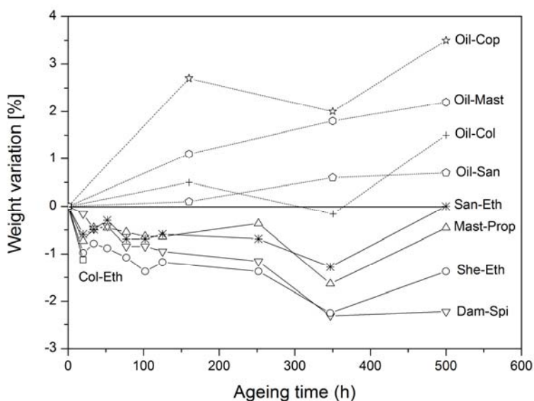
Fig. 1 - Weight variation of varnishes applied on glass as a function of ageing time.
