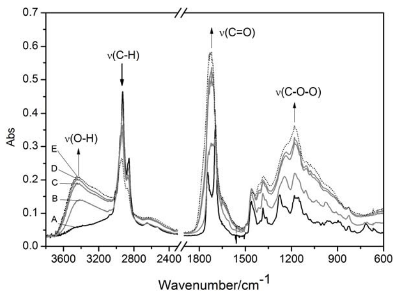
Fig. 10 Transmission FTIR spectra of Oil-Col at different ageing times (A: after 1 week. B: 0h. C: 25h. D: 50h. E: 500h). The arrows indicate the main changes observed.
