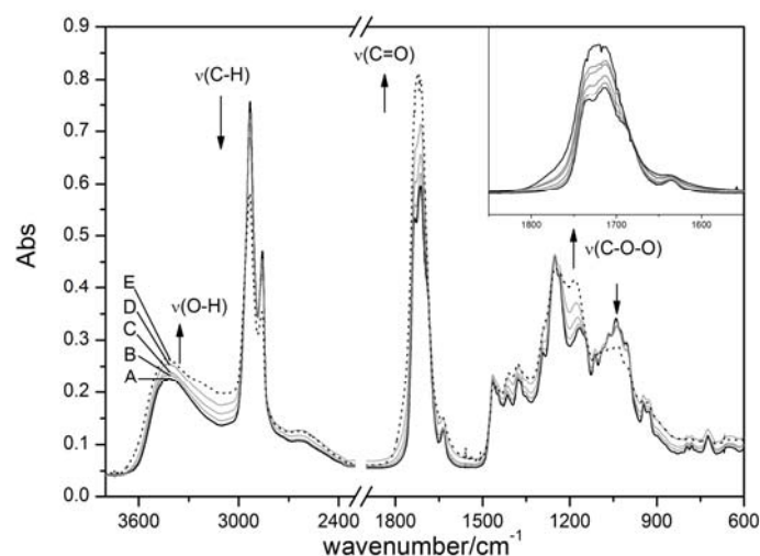
Fig. 5 Transmission FTIR spectra of She-Eth varnish film (pre-dissolved in ethanol) at different ageing times (A: 0h, B: 20h, C: 50h, D: 100h, E: 500h). The arrows indicate the changes of the main vibration groups induced by the irradiation while in the inset reports a detail of the carbonyl stretching region.
