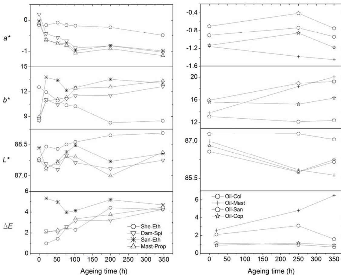
Fig.2 L^* a^* b^* coordinates and \Delta E of solvent (left) and oil (right) varnishes as function of the ageing time.
