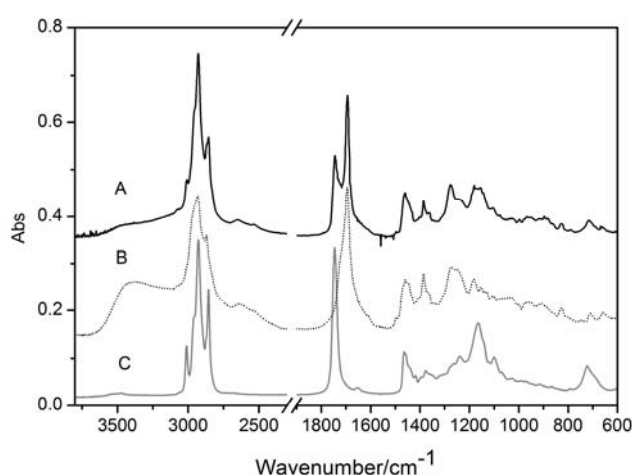
Fig. 9 Transmission FTIR spectra of Oil-Col varnish (A) after 1 week of natural curing (heated at 120^\circ\text{C} ). For a qualitative comparison fresh colophony (B) and linseed oil (C) spectra are also reported (offset).
