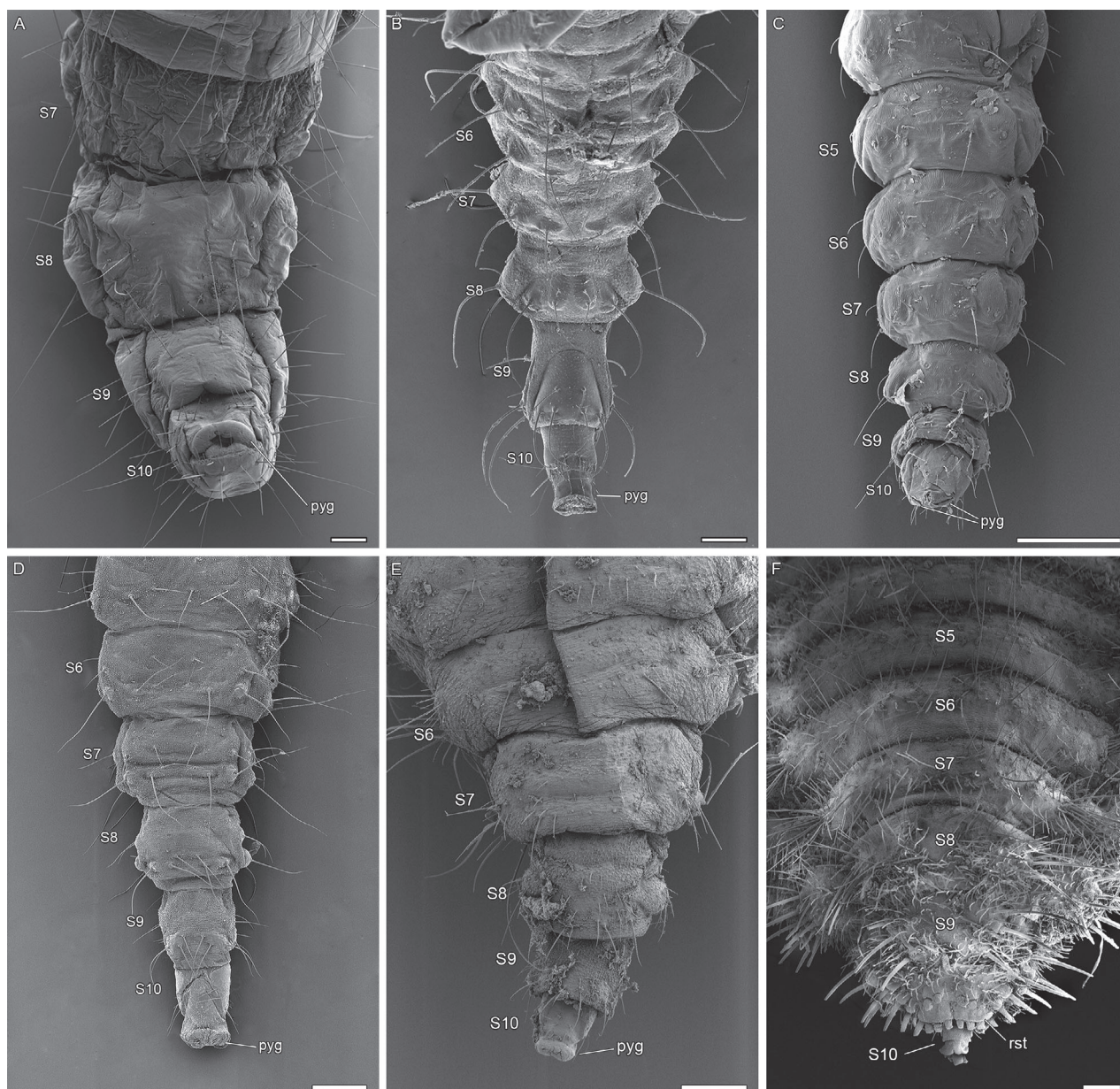
Fig. 5. Abdomen of lacewing larvae at scanning electron microscope. In ventral view: (A) Phaeostigma sp. (Raphidioptera: Raphidiidae); (B) Osmylus fulvicephalus Scopoli (Osmylidae); (C) Mantispia styriaca (Poda) (Mantispidae); (D) Hemerobius sp. (Hemerobiidae); (E) Pseudomallada sp. (Chrysopidae) and (F) Euroleon nostras Geoffroy in Fourcroy (Myrmeleontidae). Scale bar: 100 \mu m.
