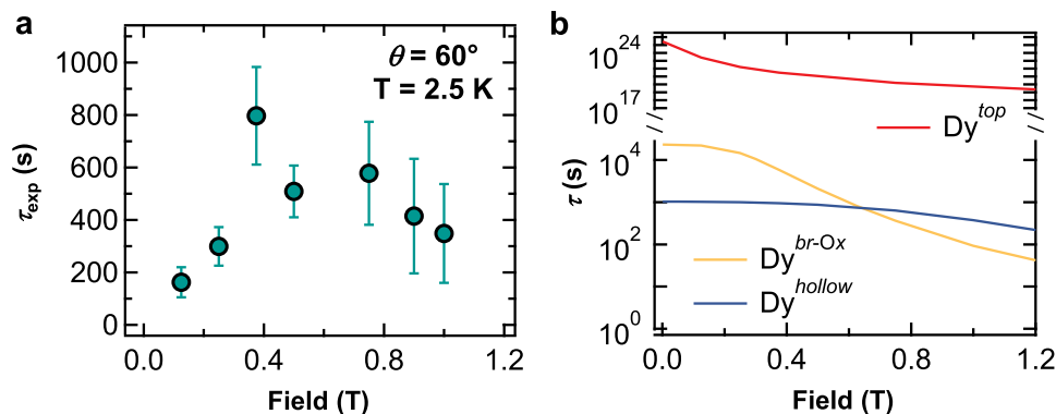
Figure 5. (a) Experimental magnetization relaxation time \tau_{\text{exp}} of Dy atoms as a function of external magnetic field B ( \Theta_{\text{Dy}} = 0.029 ML, T = 2.5 K, \theta = 60^\circ ). (b) Intrinsic relaxation time \tau calculated with the model described in the text for \text{Dy}^{\text{hollow}} , \text{Dy}^{\text{top}} , and \text{Dy}^{\text{br-Ox}} atoms ( T = 2.5 K, \theta = 60^\circ ).
