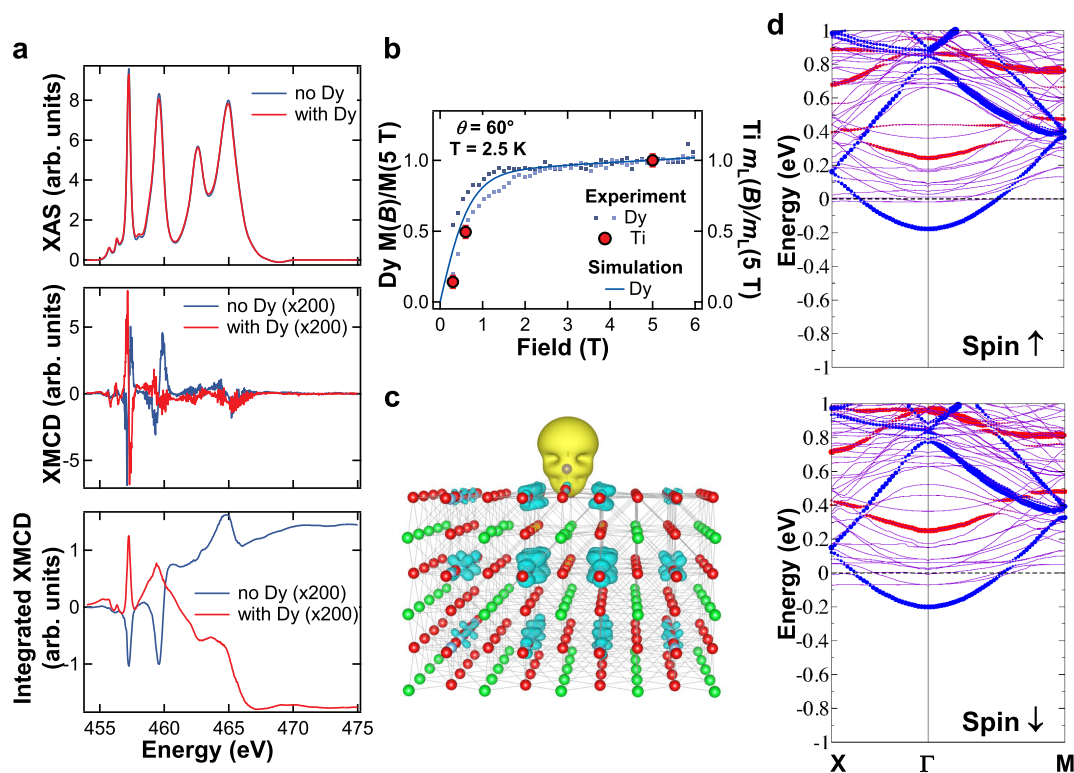
Figure 6. (a) Ti XAS (top panel) and XMCD (middle panel) spectra, with the corresponding XMCD integral (bottom panel) recorded at the L_{2,3} edges with T = 2.5 K, B = 5 T, and \theta = 60^\circ , before and after deposition of Dy ( \Theta_{\text{Dy}} = 0.035 ML) on the clean Nb:SrTiO 3 (001) surface. (b) Comparison between the magnetic field dependence of the Ti 3d orbital magnetic moment m_l (red dots) and the Dy total 4f moment (blue squares and line), both normalized at their corresponding values at B = 5 T. (c) Spin density isosurface of Dy/STO (Dy hollow sites, 4 \times 4 cell corresponding to \Theta_{\text{Dy}} = 0.06 ML, GGA, isovalue of 10^{-3} \text{ e}^-/\text{\AA}^3 ), highlighting the magnetic polarization of Ti induced by Dy. Yellow and cyan colors are associated with an excess of spin up and down electrons, respectively. (d) Spin-resolved electronic band structures (top: spin-up, bottom: spin-down) for Dy adatoms ( \Theta_{\text{Dy}} = 0.06 ML) at the hollow site of the TiO 2 terminated surface. The orbital projection on the Ti- d_{xy} character is highlighted by filled red circles (whose size is proportional to its contribution at each eigenvalue) for the surface Ti layer and by filled blue circles for the first subsurface Ti layer. The spin splitting at the \Gamma point amounts to 22 meV.
