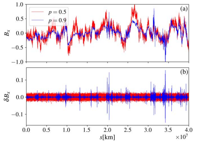
Figure 2. (a) One magnetic field component, B_x , for intermency levels p = 0.5 (red) and p = 0.9 (blue) sampled along a line s in any direction (the system is isotropic) with resolution \delta s \simeq 30 km. (b) Increments \delta B_x = B_x(s) - B_x(s + \delta s) . The field with no intermittency, p = 0.5 , does not show any “bursty” features. The field with higher intermittency ( p = 0.9 ) shows large localized spikes, an indicator of intermittency.
