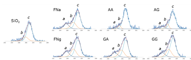
Figure 6: High resolution analysis of C1s for FNa, AA, AG, FNg, GA, GG and the substrate SiO 2 . a) 288.2 eV: O-C=O/N-
