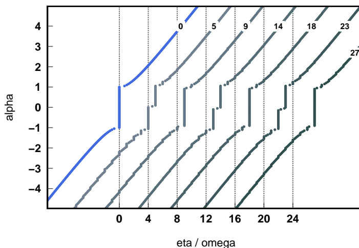
Figure 5. I - V characteristics of a junction with \beta = 0.01 for several values of \alpha_{rf} . The junction is irradiated by a train of pulses of repetition frequency \Omega = 0.45 and width \rho = 0.05 . Each curve is offset horizontally by 4\Omega and is labelled after the value of \alpha_{rf} . The vertical dotted lines mark the position of the zero-voltage axis (i.e., the critical current I_C ) for the I - V curve located immediately to the right.
